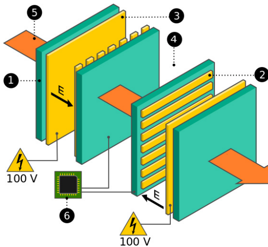
Figure 1: Schematic layout of PEPITES prototype. CP1™ membranes (1) sustain 50 nm thick gold strips (2) or are fully metallized (3). They stand in vacuum (4) where the beam (5) crosses the strips and produce secondary electrons. The signals coming from each strip are read by a dedicated readout chip (6). The final prototype will be made of 32 strips cathodes (2).
