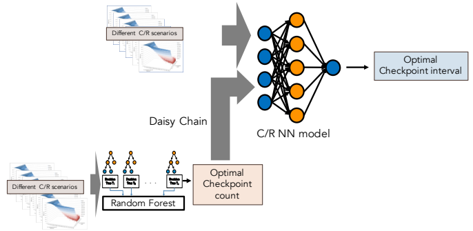
Fig. 3: Daisy Chaining output from checkpoint count prediction as an input to the neural network for checkpoint interval prediction
