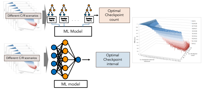
Fig. 2: Combining Simulation Approach with Machine Learning
