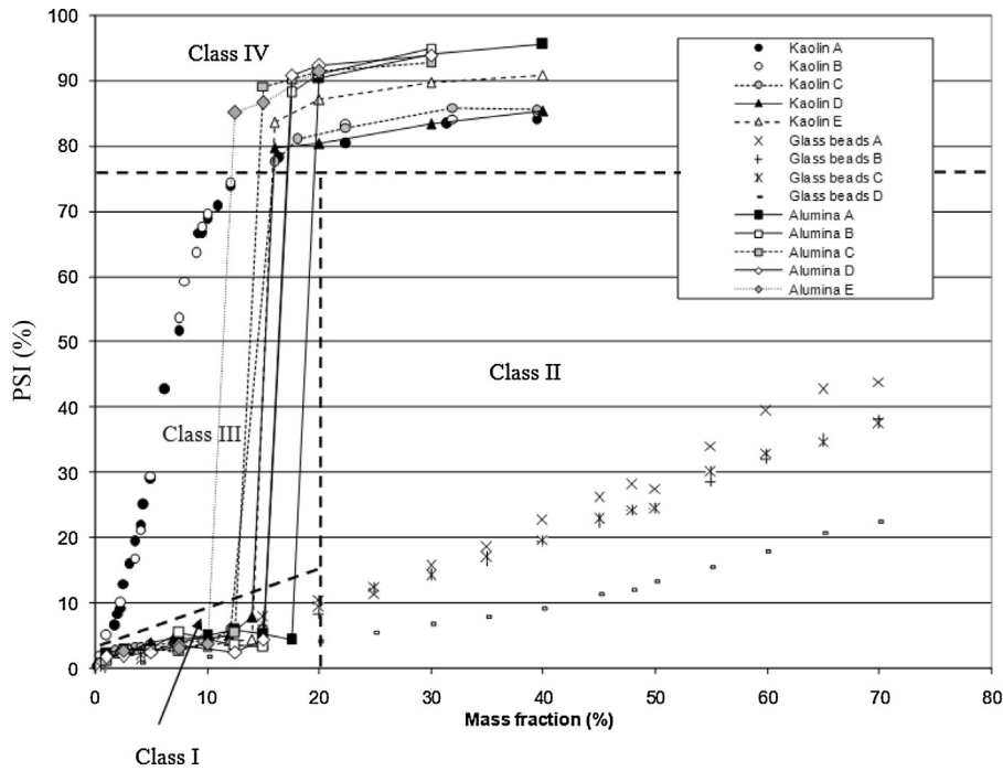
Fig. 2. Phase separation index variations as a function of mass fraction and different classes of suspension.
