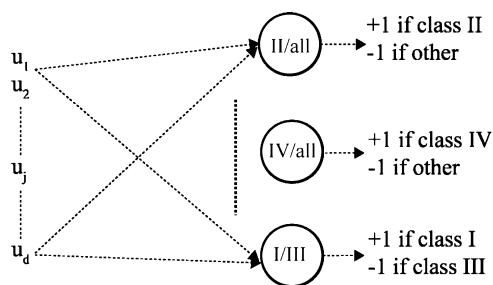
Fig. 6. Architecture of the networks inferred by the STEPNET procedure.
