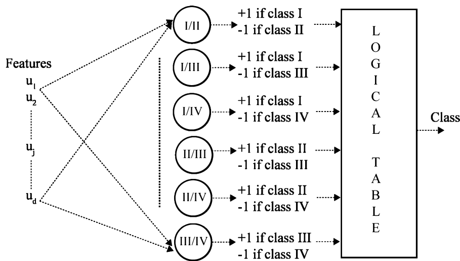
Fig. 8. Non linear classification using six linear perceptrons and a logical table.
