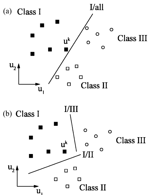
Fig. 7. (a) Linear separation from one class (I) to all others (II and III). Separation is very close to the examples and generalization could be not perfect. (b) Linear separation from one class (I) to each of others (II and III). Separations can be optimal.
