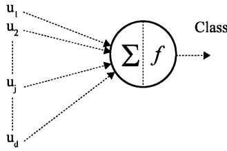
Fig. 4. A single neuron as linear classifier, f(\cdot) is the threshold function.
