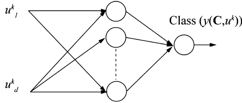
Fig. 5. Multilayer perceptron with one hidden layer and one output neuron.
