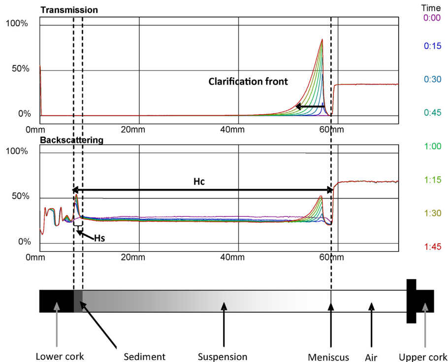
Fig. 1. Example of Turbiscan MA 2000 transmission and backscattering profiles. Determination of sedimentation column height ( H_c ) and sediment height ( H_s ).
