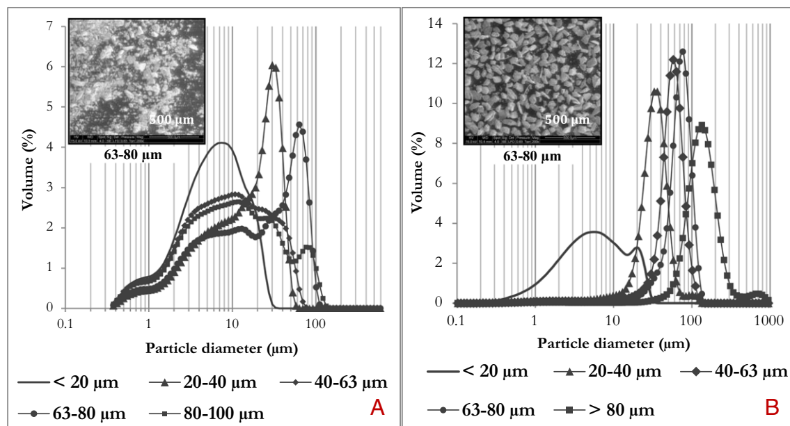
Fig. 12. Fraction particle size distributions and scanning electron micrograph of 63\text{--}80\ \mu\text{m} fraction (Ss84) obtained with A) traditional wet sieving; B) stirred sieving and rinsing.
