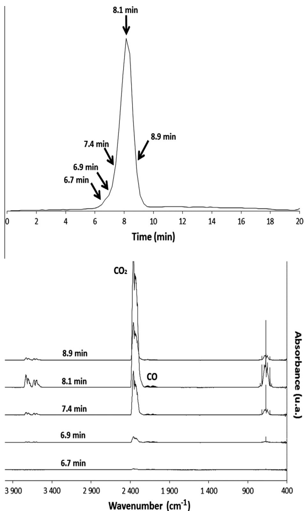
Fig. 2. Gram-Schmidt (top) and FTIR spectra (bottom) of gases after pyrolysis of LDPE and combustion at 700 °C.
