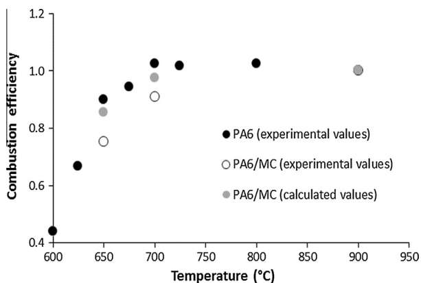
Fig. 13. Combustion efficiency versus combustion temperature for PA6 and PA6/MC blend, measured using PCFC (anaerobic pyrolysis, 1 K/s).
