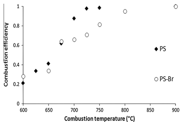
Fig. 5. Combustion efficiency versus combustion temperature for PS and PS-Br, measured using PCFC (anaerobic pyrolysis, 1 K/s).
