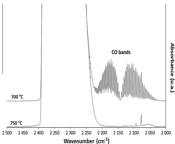
Fig. 3. Details of FTIR spectra of gases after pyrolysis of LDPE and combustion at 700 and 750 °C (at peak of heat release rate).
