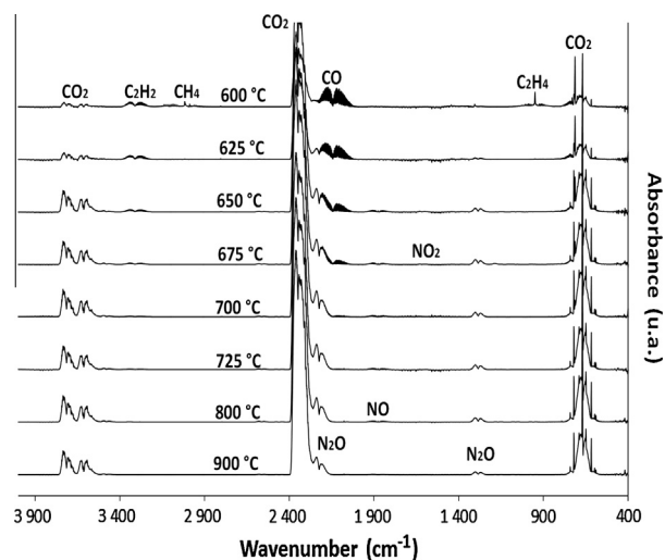
Fig. 11. FTIR spectra of gases released after pyrolysis of PA6 and combustion at various temperatures and at peak heat release rate.
