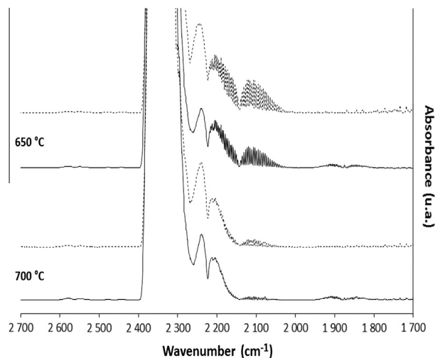
Fig. 14. FTIR spectra of gases released after pyrolysis of PA6 (solid line) and PA6/MC blend (dotted line) and combustion at 650 and 700 °C at peak heat release rate.
