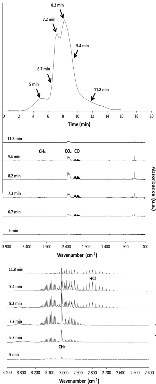
Fig. 9. Gram-Schmidt (top) and FTIR spectra (middle and bottom) of gases after pyrolysis of chloroprene and combustion at 650 °C. Arrows indicate the times of FTIR analyses.
