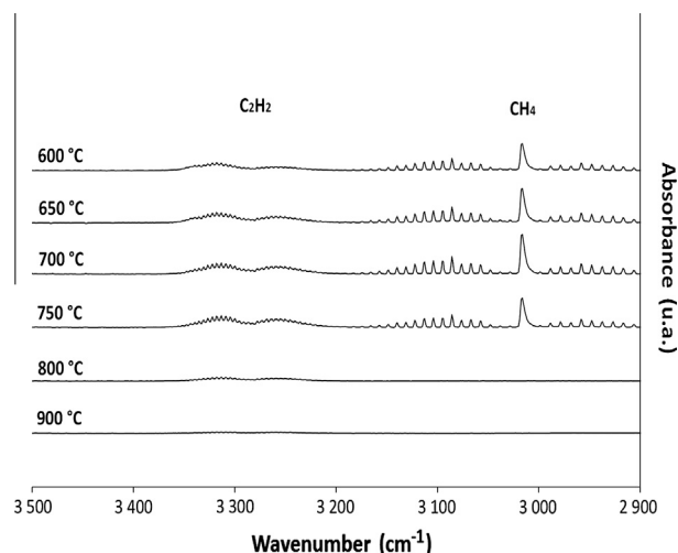
Fig. 8. Details of FTIR spectra of gases released after pyrolysis of PS-Br and combustion at various temperatures and at peak heat release rate.
