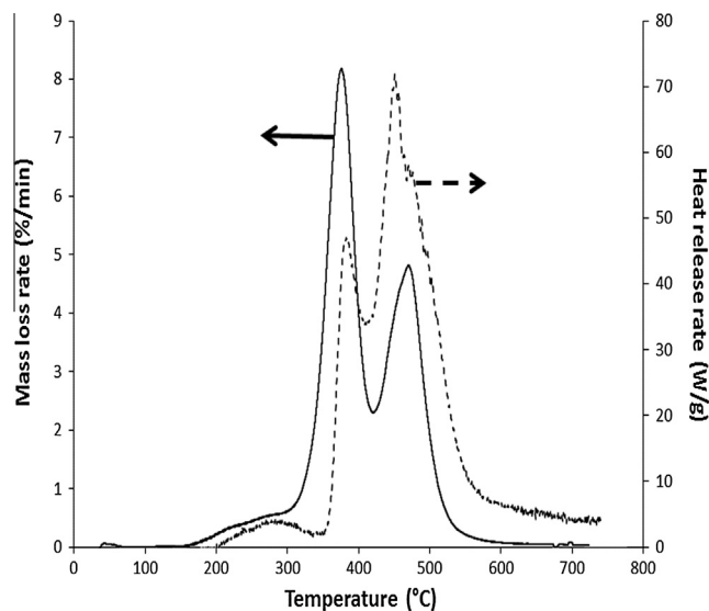
Fig. 10. Mass loss rate of chloroprene measured in TGA at 10 °C/min and heat release rate measured in PCFC at 1 K/s.
