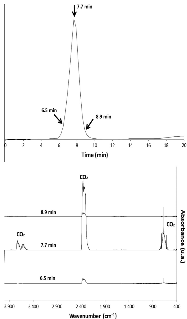
Fig. 1. Gram-Schmidt (top) and FTIR spectra (bottom) of gases after pyrolysis of LDPE and combustion at 750 °C.
