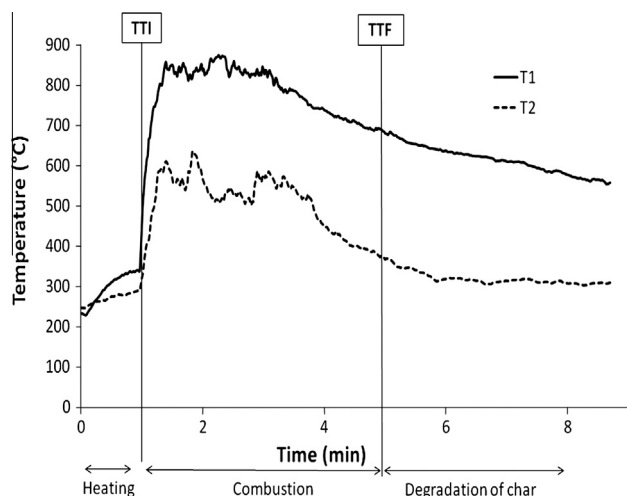
Fig. 17. Temperatures obtained by two thermocouples during the cone calorimeter test (without spark igniter). TTI: time to ignition.
