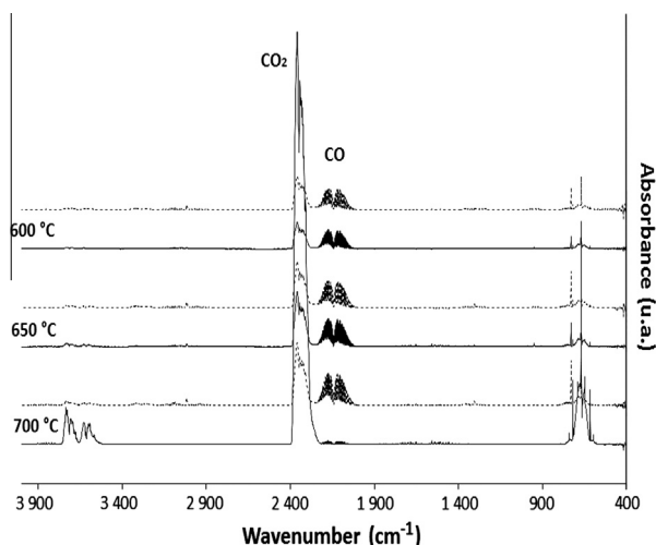
Fig. 6. FTIR spectra of gases released after pyrolysis of PS (solid line) and PS-Br (dotted line) and combustion at various temperatures and at the peak heat release rate.
