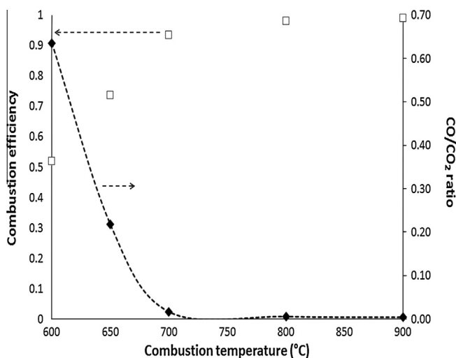
Fig. 18. Combustion efficiency and CO/CO 2 ratio versus the temperature of combustion for cellulose, measured using PCFC (anaerobic pyrolysis, 1 K/s).
