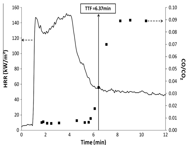
Fig. 15. HRR versus time at an irradiance of 35 kW/m 2 (—) and a CO/CO 2 ratio obtained during the cone calorimeter test (■).
