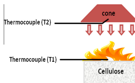
Fig. 16. Position of thermocouples in the combustion zone during the cone calorimeter test.
