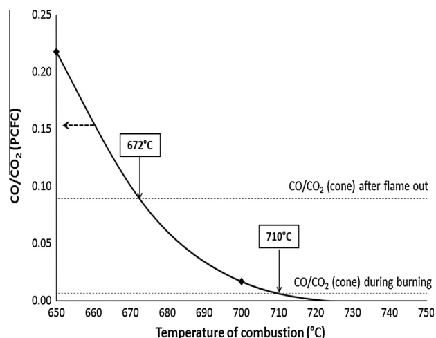
Fig. 19. Comparison of CO/CO 2 ratio obtained in FTIR-cone calorimeter and FTIR-PCFC coupling.
