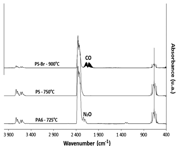
Fig. 4. FTIR spectra of gases after pyrolysis of PA6, PS, and PS-Br and combustion at 725, 750, and 900 °C, respectively.
