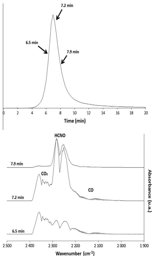
Fig. 12. Gram-Schmidt (top) and FTIR spectra (bottom) of gases after pyrolysis of melamine cyanurate and combustion at 900 °C.
