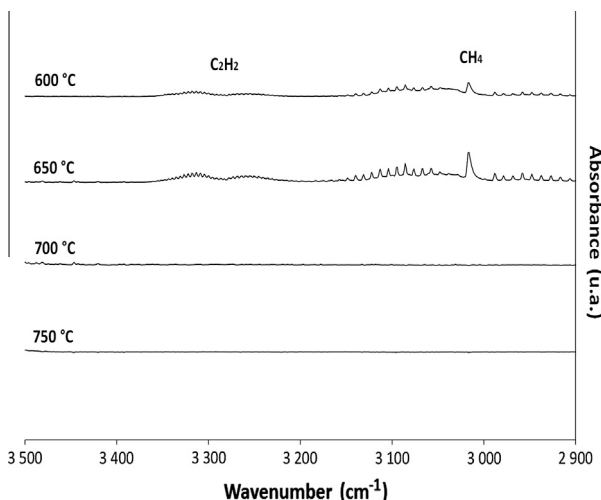
Fig. 7. Details of FTIR spectra of gases released after pyrolysis of PS and combustion at various temperatures and at peak heat release rate.
