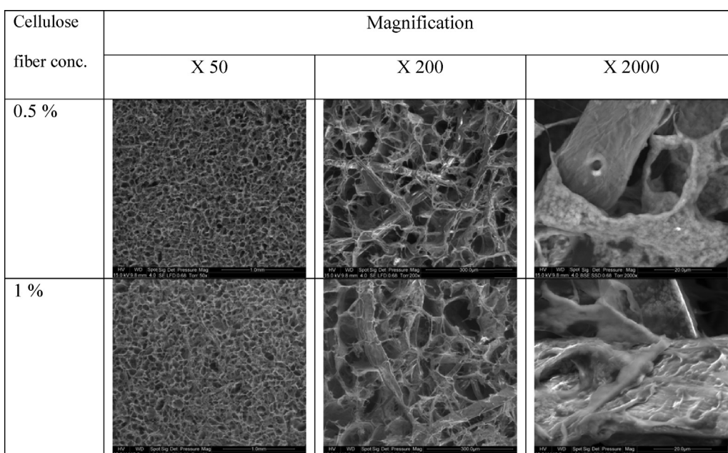
Fig. 4. SEM analysis of chitin-PB composite sponges with inclusion of cellulose fibers (at different loads, 0.5% and 1% of the solution mixture) at different magnifications (Secondary electrons detection).
