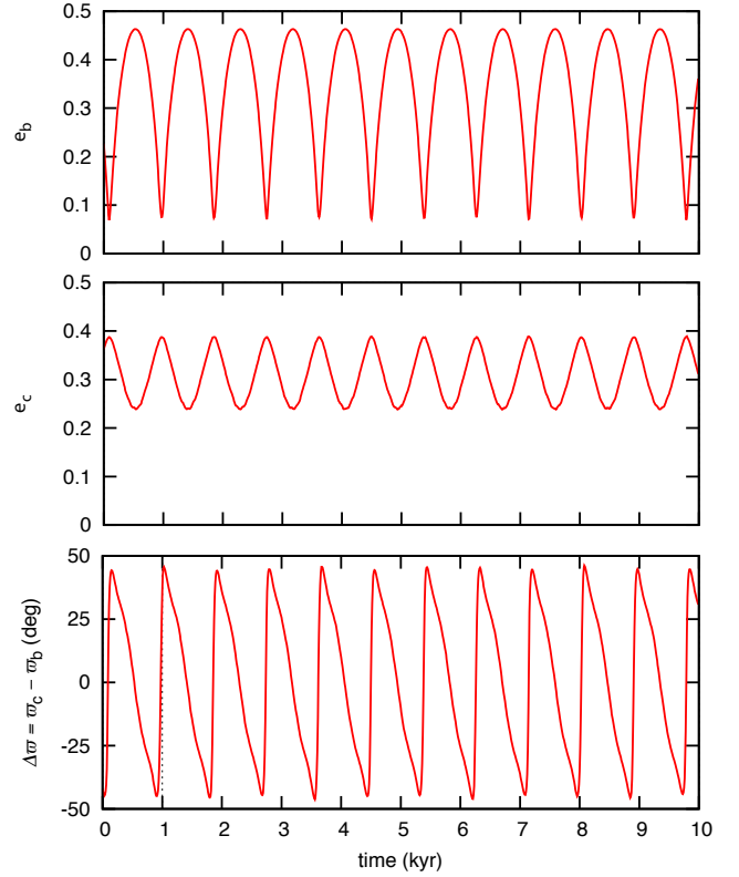
Fig. 8. Secular evolution of the WASP-148 system, assuming coplanar orbits (Table 6). We show the eccentricity of WASP-148b (top) and WASP-148c (middle), and the angle \Delta\omega = \omega_c - \omega_b (bottom). These three parameters oscillate with an 881 yr period.
