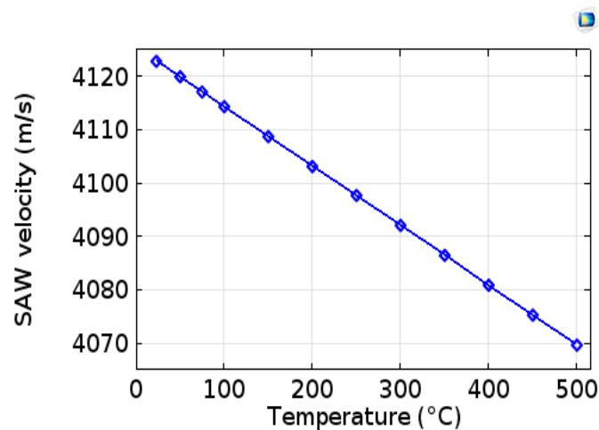
Figure 6. Variation in Rayleigh velocity as a function of temperature.
