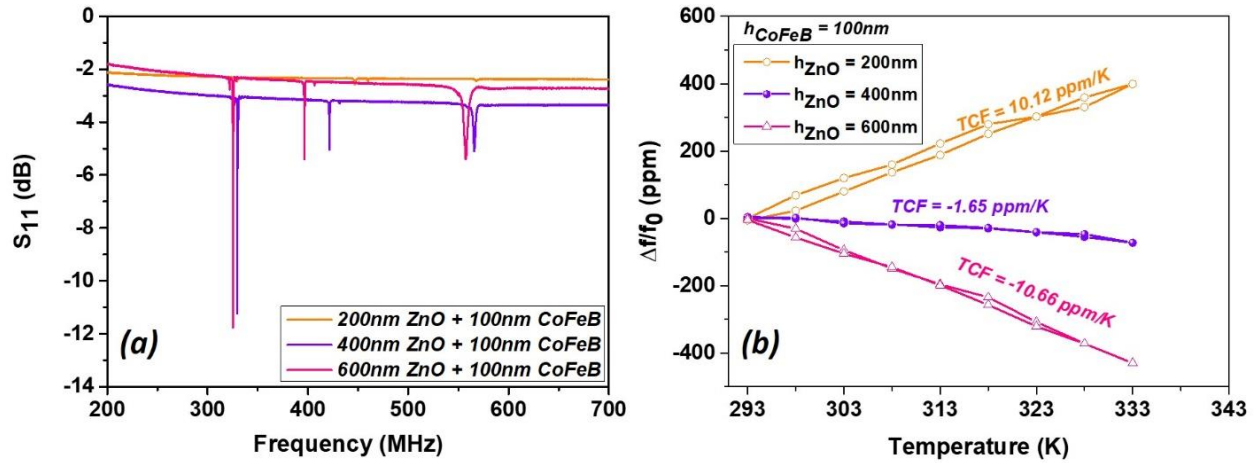
Figure 4: (a) Scattering parameter ( S_{11} ) measured on samples with different ZnO thicknesses after deposition and micro-structuration of 100nm of CoFeB; (b) TCF measured on the Love wave resonances in the three devices.
