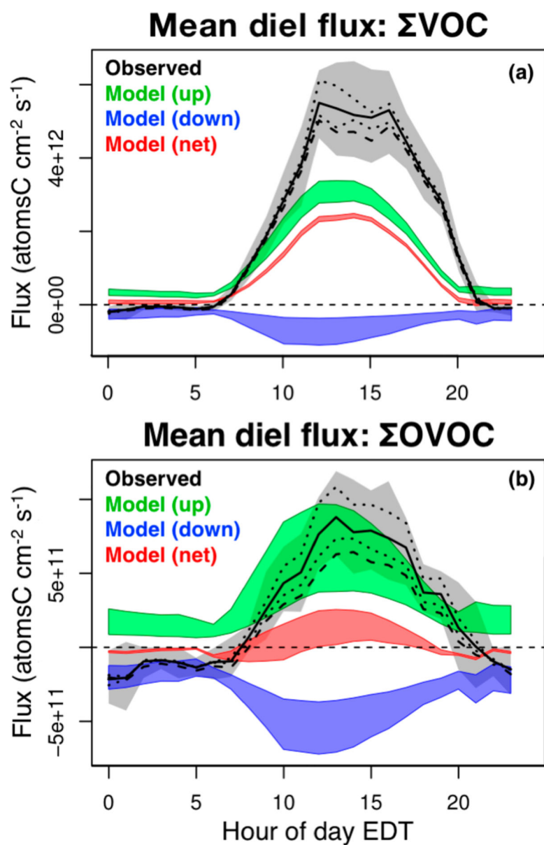
Figure 5. Mean diel cycle of forest–atmosphere fluxes for the sum of all VOCs ( \Sigma VOC, panel a) and the sum of all oxygenated VOCs ( \Sigma OVOC, panel b). The black solid line and shaded gray region show the mean observed flux and associated 95% confidence interval. Dotted lines show results using upper and lower sensitivity assumptions for uncalibrated compounds as described in-text. The dashed line shows the mean observed diel cycle for the VOC subset that is explicitly included in the GEOS-Chem CTM. Green, blue, and red regions span upper and lower limits for the model-derived gross upward, gross downward, and net fluxes as described in-text.
