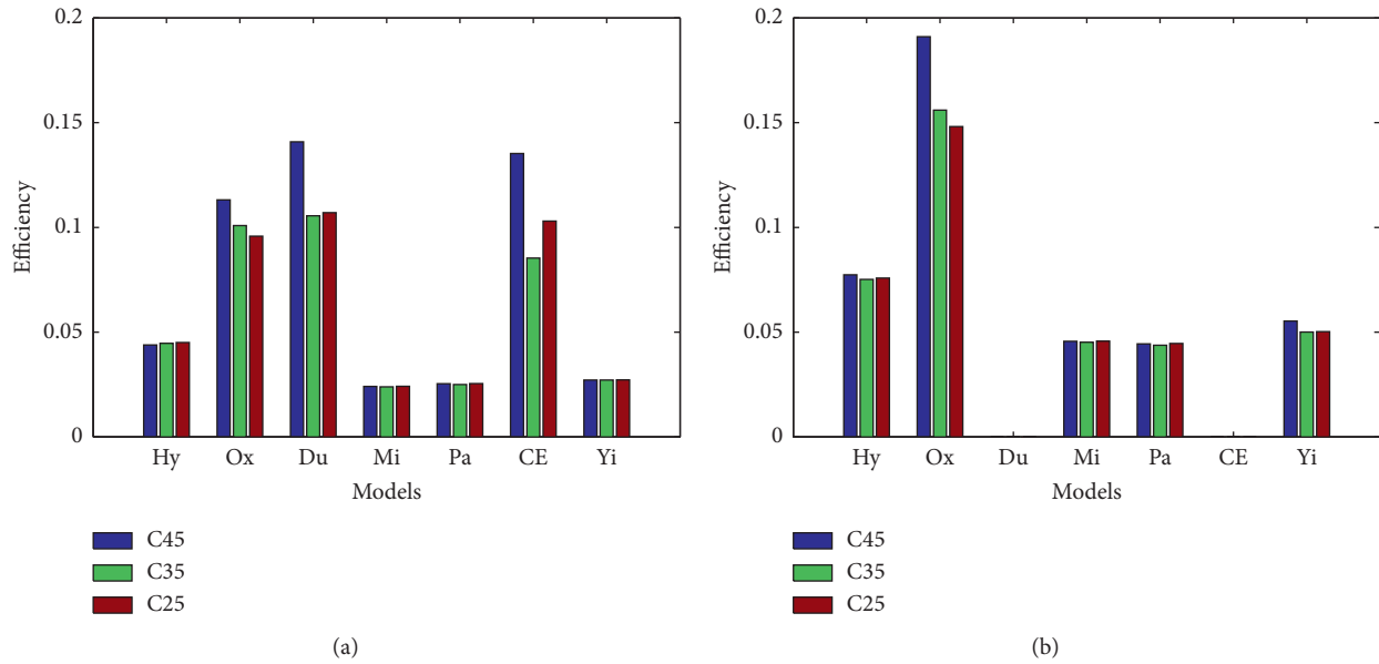
FIGURE 7: Efficiency of each concrete carbonation model when applied to concretes C45, C35, and C25 for structure A (a) and for structure B (b).
