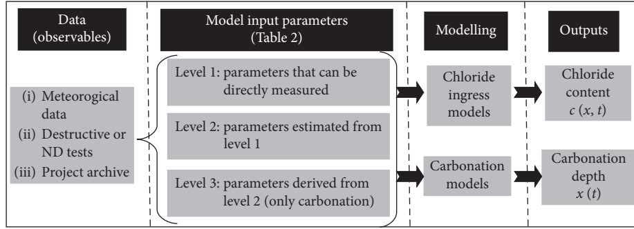
FIGURE 2: General representation of input parameters for analytical carbonation and chloride ingress models by Rakotovoav Ravahatra et al. [17].
