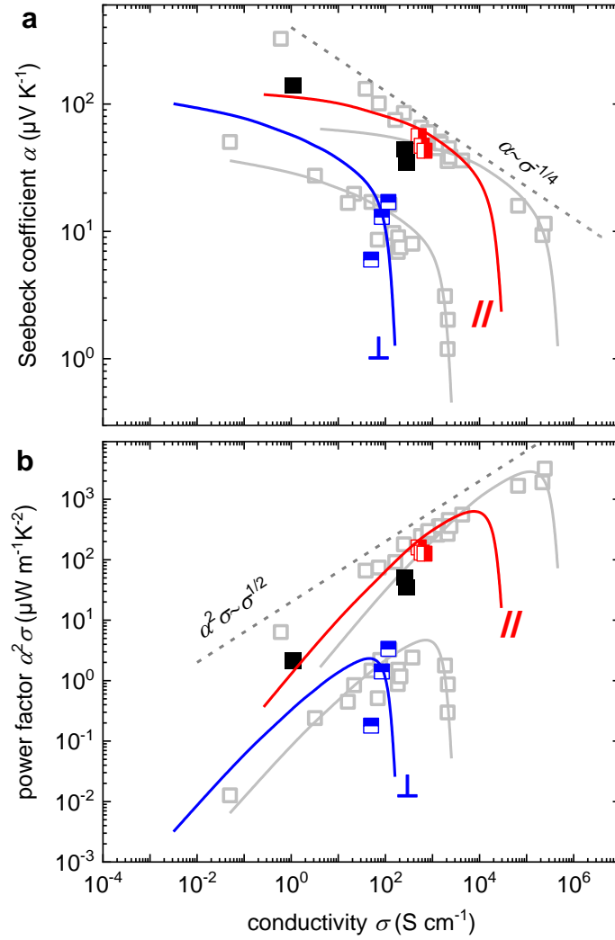
Figure 4. (a) Seebeck coefficient \alpha and (b) power factor \alpha^2\sigma versus electrical conductivity \sigma of isotropic P3HT (black squares), and rubbed P3HT measured parallel (red squares and line) and perpendicular to the rubbing direction (blue squares and line); grey data points are literature values extracted from refs. 9, 38 for PBTTT. Full lines correspond to simulations calculated from the kMC model, with an anisotropy ratio of \xi_{\parallel}/\xi_{\perp} = 4 , where \xi is the localization length in the parallel and perpendicular direction, respectively. The attempt to hop frequency was set to \nu_0 = 2 \cdot 10^{13} \text{ s}^{-1} and the thermopower was rescaled by a factor of 0.1 in both directions. \parallel and \perp refer to the parallel and perpendicular direction, respectively. The dashed gray line shows the empirical trends \alpha \propto \sigma^{-0.25} and \alpha^2\sigma \propto \sqrt{\sigma} .
