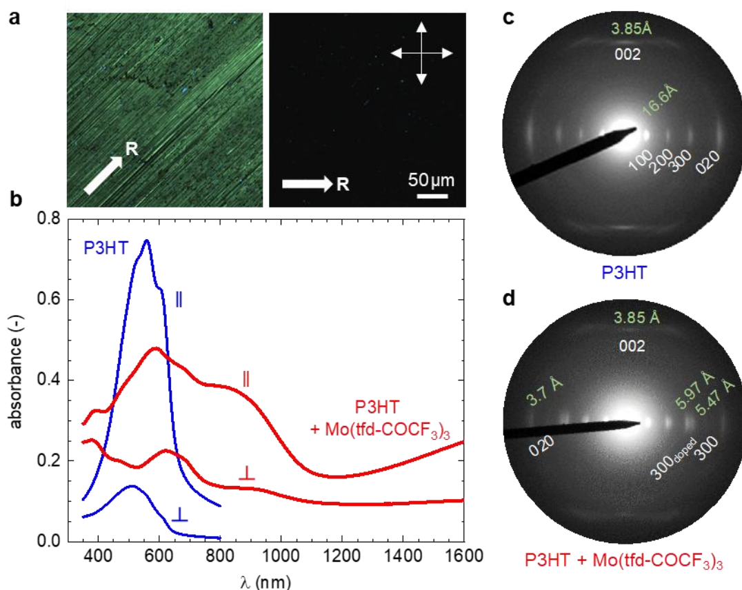
Figure 3. (a) Polarized optical microscopy images of rubbed P3HT films sequentially doped with c_{Mo} \sim 1 \text{ g L}^{-1} ; crossed double arrows indicate the orientation of polarizer and analyzer; white arrow indicates the rubbing direction R; (b) polarized UV-vis-NIR absorbance spectra of rubbed P3HT and the same P3HT film doped with c_{Mo} \sim 1 \text{ g L}^{-1} measured parallel (||) and perpendicular ( \perp ) to the rubbing direction R; (c, d) electron diffraction patterns of neat rubbed P3HT and rubbed P3HT doped with \text{Mo}(\text{tfd-COCF}_3)_3 .
