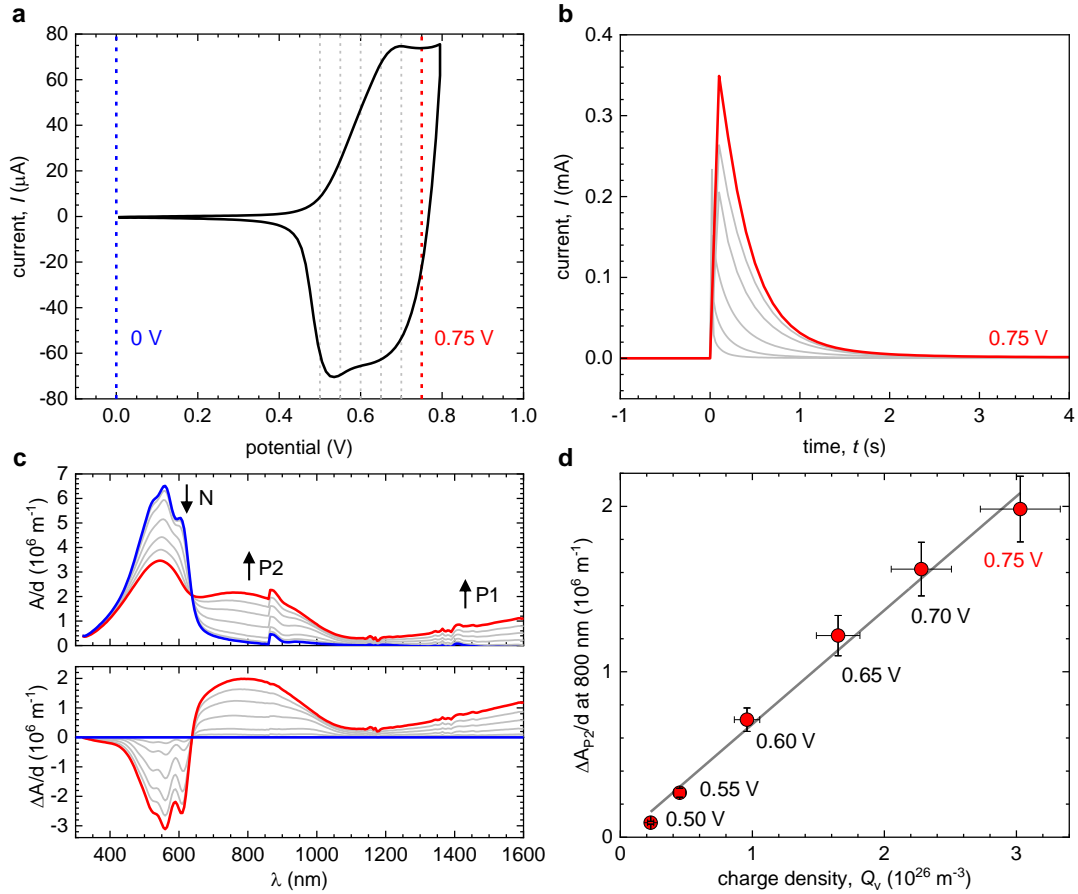
Figure 2. (a) Cyclic voltammogram of P3HT (P3HT has an oxidation onset around 0 V vs. ferrocene/ferrocenium according to ref. 28); (b) charging current from chronoamperometry, (c) UV-vis-NIR absorbance spectra from spectroelectrochemistry measurements recorded at different electrochemical potentials between 0 V (blue) and 0.75 V (red); thickness normalized absorbance A/d (top) and difference in normalized absorbance \Delta A/d between spectra of P3HT oxidized at different potentials and undoped P3HT at 0 V; (d) the differential absorbance \Delta A_{P2}/d at 800 nm vs. charge density Q_v from integration of the charging currents; the slope of the linear fit (gray) is the molar attenuation coefficient \epsilon_{P2} .
