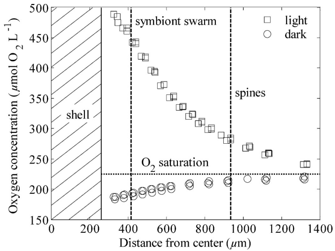
Fig. 1. Oxygen gradients observed in triplicates for O. universa at 29.3°C in light and dark conditions. Vertical dashed line indicates the outer periphery of the symbionts swarm and of the spines. Horizontal dashed line indicates the 100% O_2 saturation.
