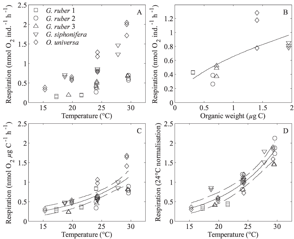
Fig. 2. Respiration rate of G. ruber , G. siphonifera , and O. universa . (A) Respiration rate ( \text{nmol } O_2 \text{ ind.}^{-1} \text{ h}^{-1} ) in relation to temperature. (B) Respiration rate at 24°C in relation to the organic weight ( \mu\text{g C} ) calculated from shell size and a conversion factor from Michaels et al. (1995). Continuous line: least-squares regression for data fitted with a power model with a 0.57 \pm 0.18 exponent. (C) Respiration rate in relation to temperature of the different specimens calculated for a 1 \mu\text{g C} individual using the precedent relationship (panel B). (D) Respiration rate in relation to temperature of the different specimens normalized by the mean observed value at 24°C. Solid line: least-squares regression for data fitted with the Arrhenius relationship (Table 2); dashed lines: 95% confidence intervals for the regression.
