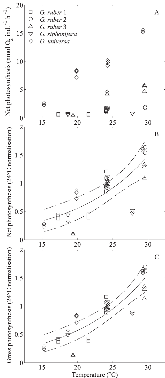
Fig. 3. Photosynthesis rate of G. ruber , G. siphonifera , and O. universa . (A) Net photosynthesis rate ( \text{nmol O}_2 \text{ ind.}^{-1} \text{ h}^{-1} ) in relation to temperature. (B) Net photosynthesis rate in relation to temperature of the different specimens normalized by the mean observed value at 24^\circ\text{C} . (C) Gross photosynthesis rate in relation to temperature of the different specimens normalized by the mean observed value at 24^\circ\text{C} . Solid lines: least-squares regression for data fitted with the Arrhenius relationships (Table 2); dashed lines: 95% confidence intervals for the regression.
