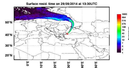
Figure 2. Surface residence time of representative air mass trajectories from the FLEXPART model during the TRANSEMED Istanbul campaign.
