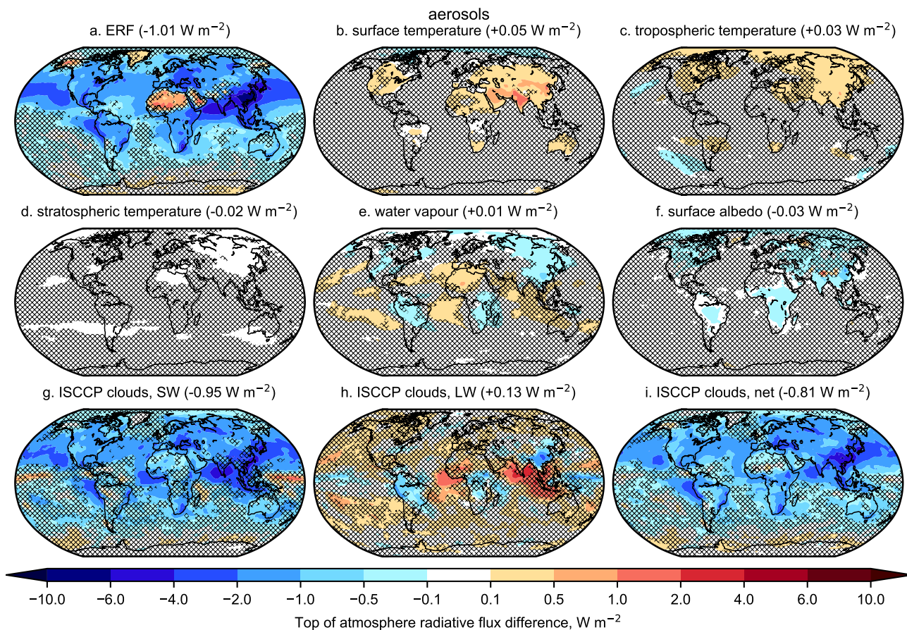
Figure 8. As fig. 6 but for present-day aerosol forcing.
