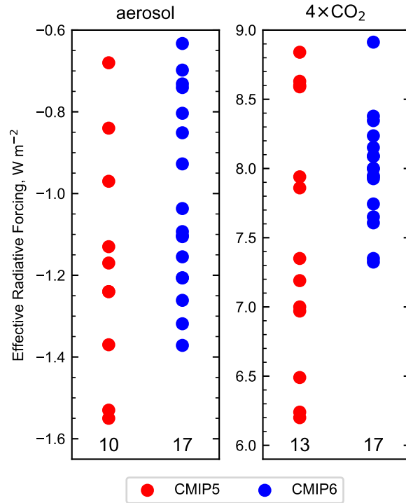
Figure 5. Aerosol and 4\times\text{CO}_2 effective radiative forcing from CMIP5 sstClim4xCO2 and sstClimAerosol experiments (Kamae and Watanabe, 2012; Zelinka et al., 2014) and CMIP6 RFMIP experiments. Numbers at the bottom of each plot give the number of participating models.
