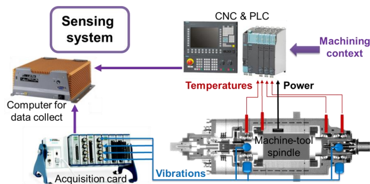
Figure 6. In-process data collection system
