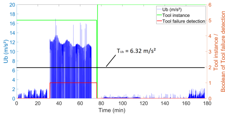
Figure 12. Visualization of U_b criterion (in blue) for tool reference 36, the index of tool instance (in green) and the Boolean for tool failure detection (in red).
