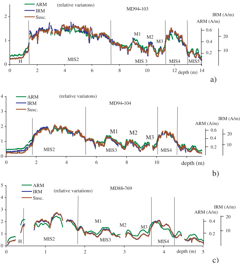
Figure 4. Variations of the low field susceptibility ( \kappa ), ARM, and IRM obtained for the 3 cores: (a) MD94-103, (b) MD94-104, and (c) MD88-769.
