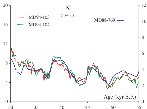
Figure 8. The susceptibility records obtained for the 3 cores during MIS3 after correlating cores MD94-104 and MD88-769 to core MD94-103.
