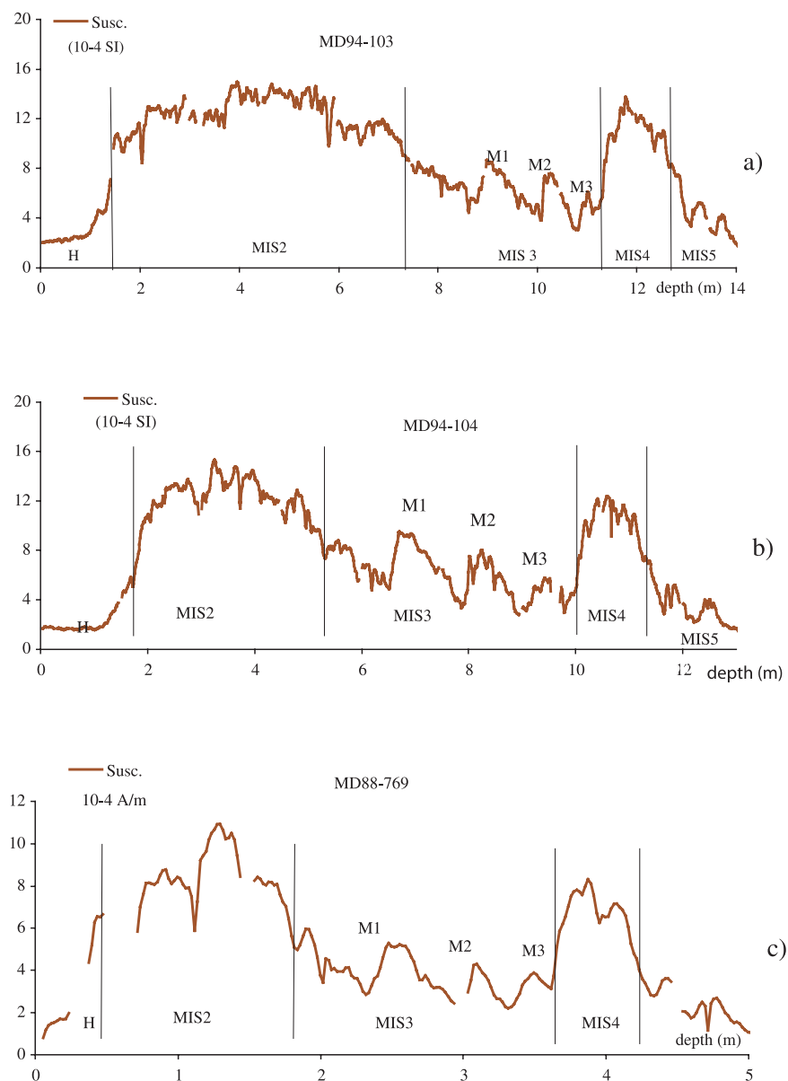
Figure 3. Low field susceptibility ( \kappa ) measured at high resolution for the 3 cores: (a) MD94-103, (b) MD94-104, and (c) MD88-769. Positions of the Marine Isotopic Stages as identified by Dezileau et al. [2000] are also indicated.
