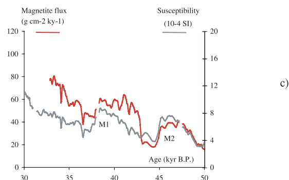
Figure 10. (a) Percentage of \text{CaCO}_3 in core MD94-103, (b) low field susceptibility before and after carbonate detrending, and (c) magnetite flux calculated for core MD94-103 in the 30–50 kyr B.P. interval.
