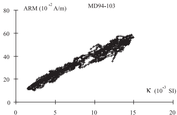
Figure 5. ARM plotted against \kappa .
