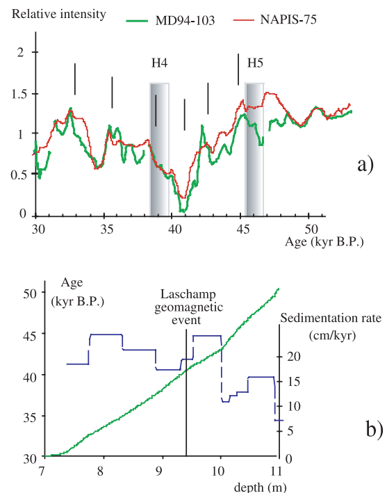
Figure 7. (a) Correlation of core MD94-103 geomagnetic intensity record to the NAPIS-75 stack (figure from Mazaud et al. [2002]). The tie points are indicated by vertical lines. The Laschamp geomagnetic event corresponds to the geomagnetic intensity low at \approx 41 kyr B.P. (b) Age model of core MD94-103 and derived accumulation rate.
