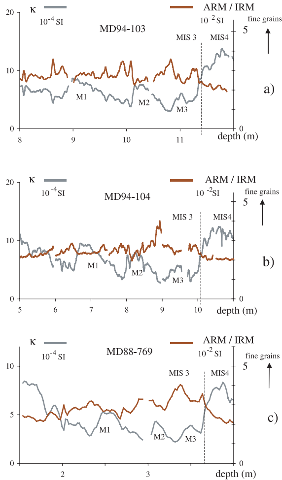
Figure 6. Variations of ARM/IRM and \kappa obtained for three cores: (a) MD94-103, (b) MD94-104, and (c) MD88-769.
