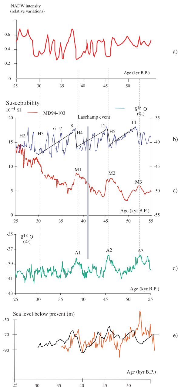
Figure 11. (a) Past variations in the 30–50 kyr B.P. of the NADW (figure after Laj et al. [2002]), (b) GISP2 isotopic record [ Grootes and Stuiver , 1997], (c) magnetic mineral concentration eastward of the Kerguelen plateau, (d) Byrd isotopic record, and (e) the sea level (orange curve: Siddal et al. [2003]; dark curve: Arz et al. [2006]). All records are placed on the GISP2 age model. The “Bond” cycles are indicated by the gray lines in the GISP2 isotopic record [see also Bond et al. , 1993].
