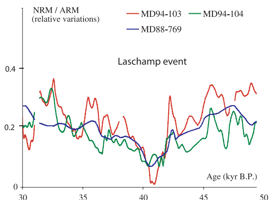
Figure 9. Relative paleointensity records obtained after correlating the susceptibility records of cores MD94-104 and MD88-769 to that of core MD94-103.
