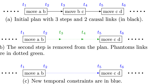
Fig. 11 Use of phantom elements on an example.
