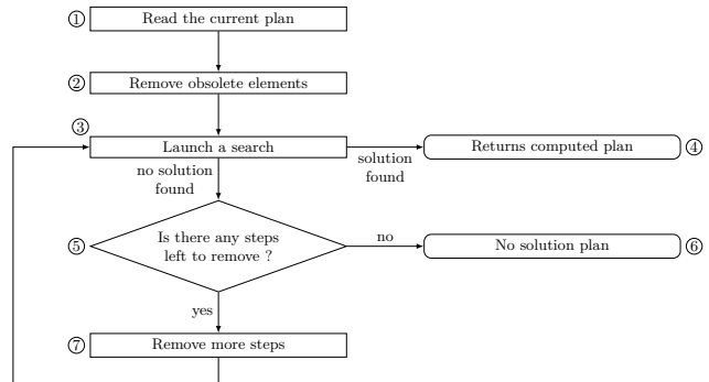
Fig. 10 Repair algorithm: the idea is to iteratively try a search starting from a partial plan computed from the initial plan until a solution is found or until the replanning fails.
