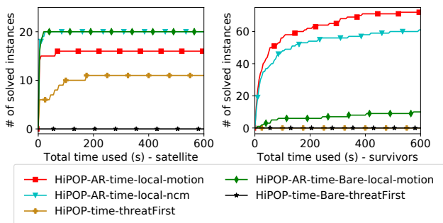
Fig. 4 Results of several configurations of HiPOP on 2 different domains. Each graph shows the number of solved problems (in the y-axis) in less than a given time (in the x-axis). The AR stands for advance reuse (see 4.2.3), the R stands for reuse . Local states that the algorithm selects first the open link for the action most recently introduced in the plan (taken from VHPOP) whereas threatFirst does not sort them: they are taken in LIFO order. motion states that geometrical reasoning is used (introduced in 4.3) and ncm stands for no cost motion . Bare means that HiPOP is not taking the abstract actions in consideration when planning: it is equivalent to a POP algorithm.
