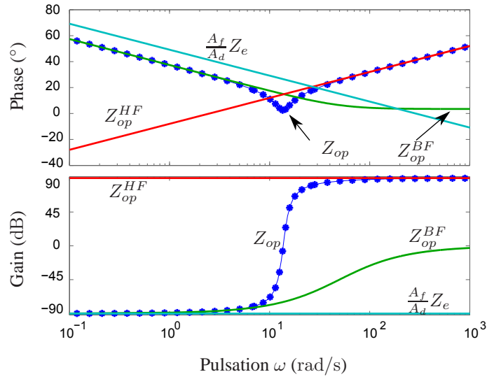
(a) mode contact
