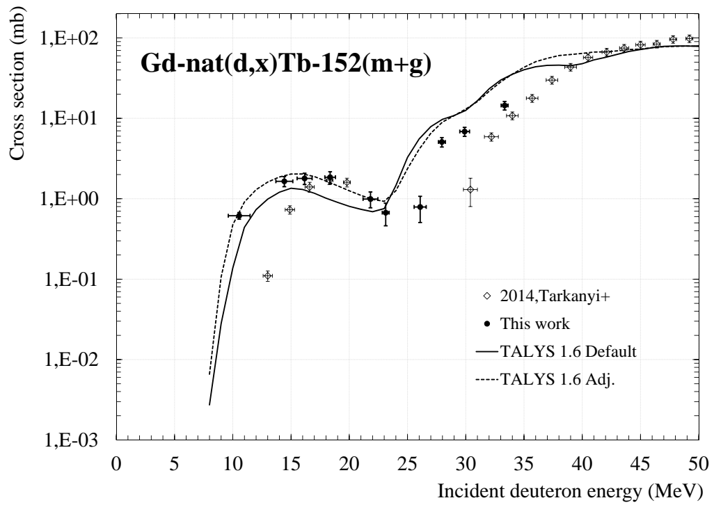
Figure 3: experimental cross section of Gd-nat(d,x)Tb-152.
