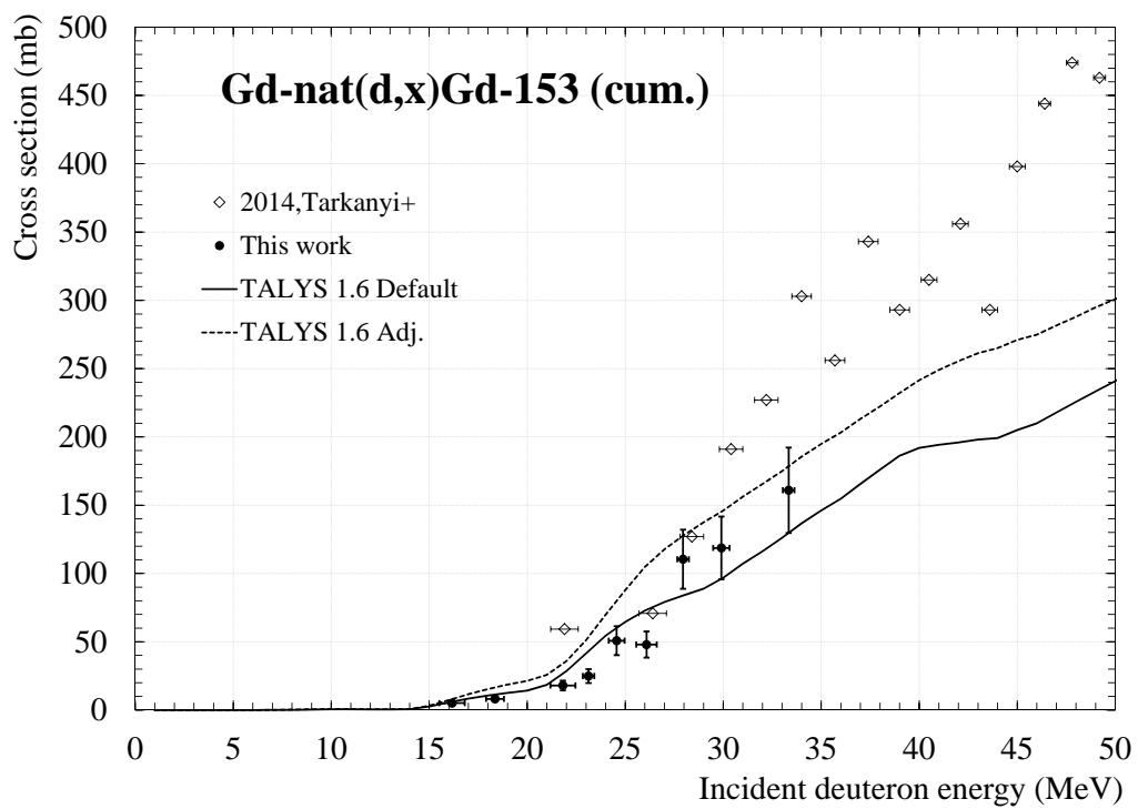
Figure 9: experimental cross section of Gd-nat(d,x)Gd-153.
