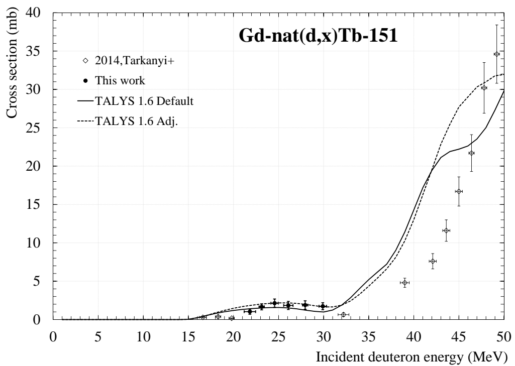
Figure 2: experimental cross section of Gd-nat(d,x)Tb-151.
