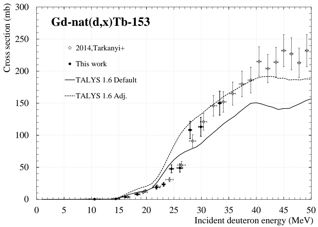
Figure 4: experimental cross section of Gd-nat(d,x)Tb-153.
