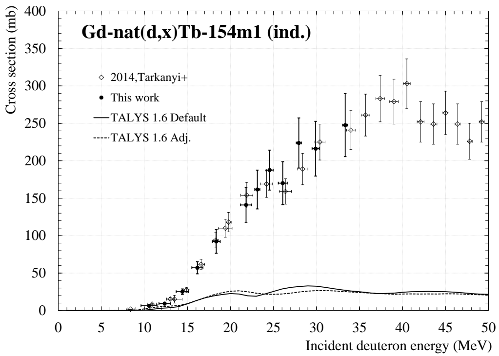
Figure 5: experimental cross section of Gd-nat(d,x)Tb-154m1.
