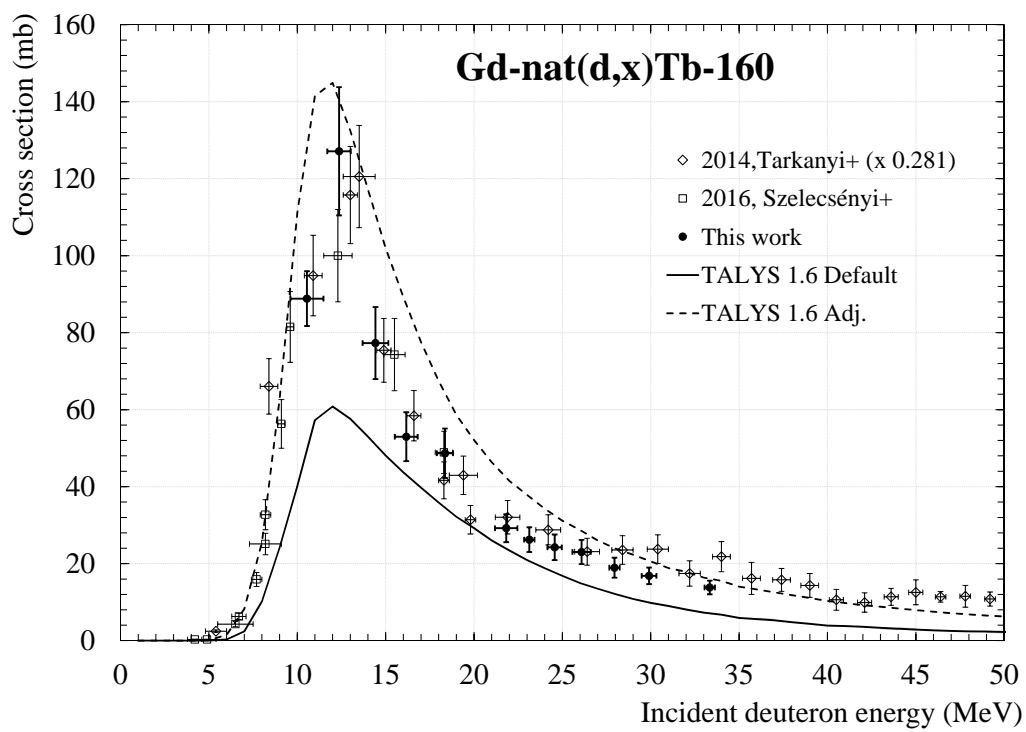
Figure 8: experimental cross section of Gd-nat(d,x)Tb-160.
