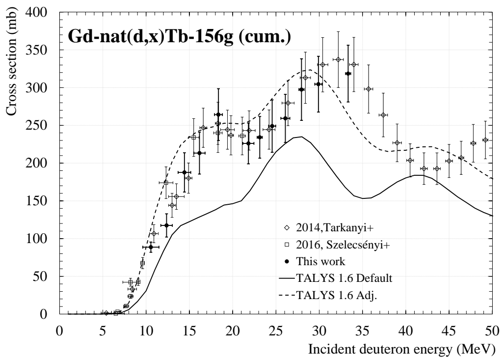
Figure 7: experimental cross section of Gd-nat(d,x)Tb-156g.
