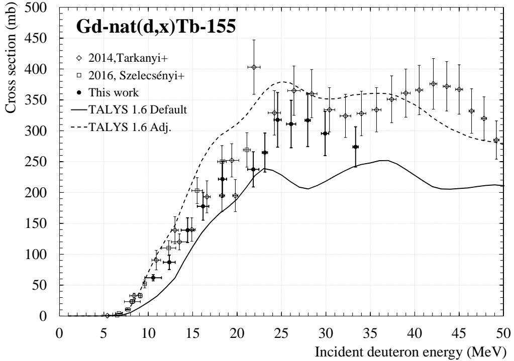
Figure 1: experimental cross section of Gd-nat(d,x)Tb-155
