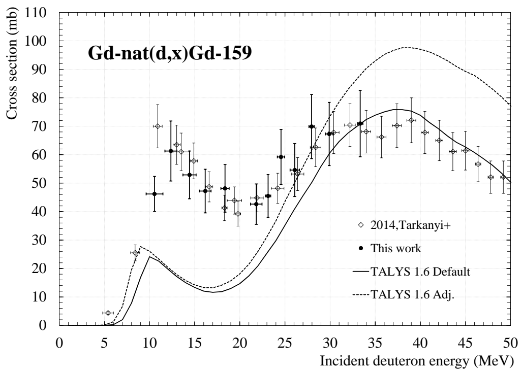
Figure 10: experimental cross section of Gd-nat(d,x)Gd-159.
