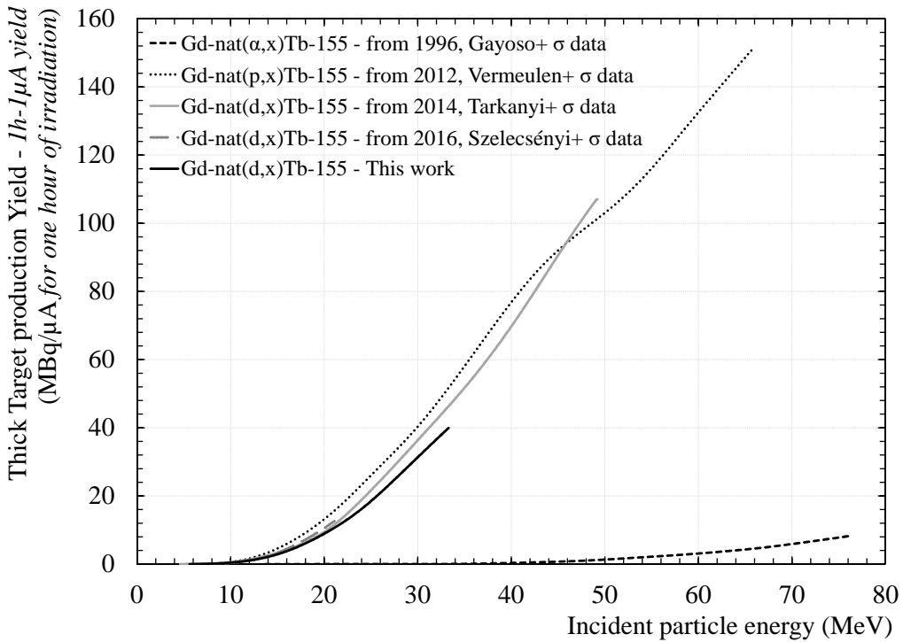
Figure 12: Tb-155 production yield comparison between proton, deuteron and \alpha particle as projectile on Gd-nat.
