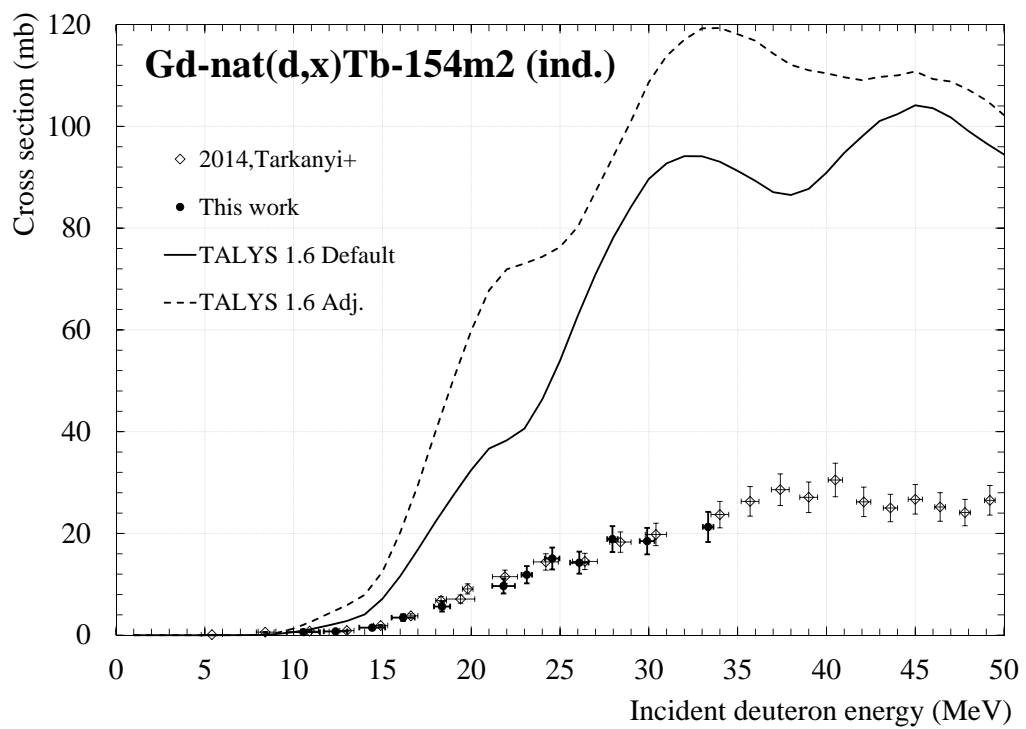
Figure 6: experimental cross section of Gd-nat(d,x)Tb-154m2.
