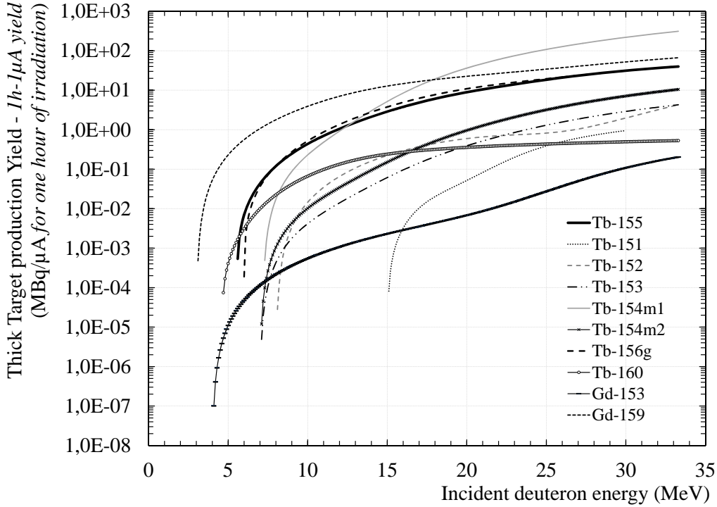
Figure 11: production yields calculated for 1 \mu\text{Ae} and 1 hour of irradiation, from our experimental cross section values obtained for the \text{Gd-nat}(d,x) reaction.
