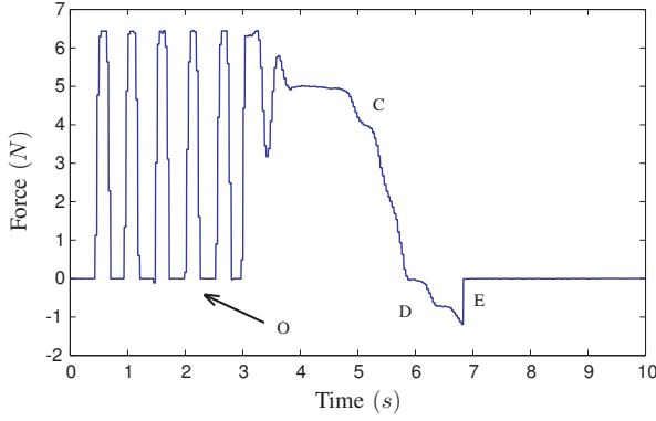
Fig. 7. Approach-retract curve for a cantilever of stiffness k_c = 2.4 \text{ N.m}^{-1} , using A_d = 0.05 \cdot 10^6 , A_f = 6 \cdot 10^6 , R=120 .
