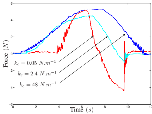
Fig. 10. Approach-retract curve for cantilevers of stiffnesses k_c = \{0.05, 2.4, 48\} N.m^{-1} ( K_{fp} = \{100, 100, 100\} N.m^{-1} , B_{fp} = \{1.2, 2.0, 1.5\} N.s.m^{-1} , G_n = \{2329, 47.5, 1.98\} m.N^{-1}.s^{-1} ).
