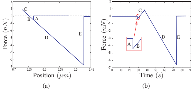
Fig. 1. Approach-retract curve
