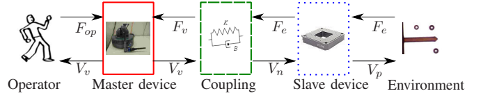
Fig. 4. Power flow between the subsystems
