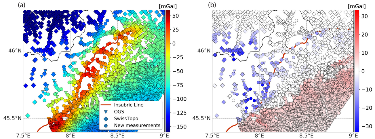
Figure 5. (a) Point-wise Bouguer gravity anomaly (BA), computed from the currently available merged gravity dataset. (b) Point-wise Niggli correction (NC), computed by taking into account mapped surface rock-densities in the terrain correction, as described in the text. This Niggli correction is negative in areas of denser rocks at the surface, and positive in areas of lighter rocks at the surface.
