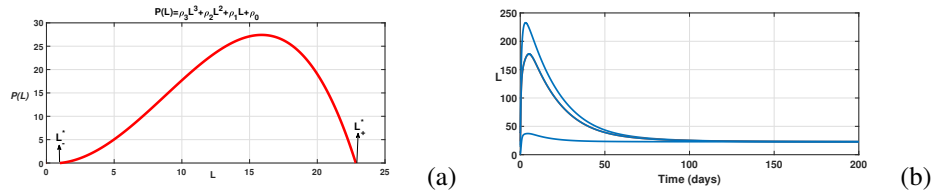
Figure 2 – Illustration of theorem 3 for 1 < \mathcal{N}^* = 61.4689 > \mathcal{N}_c = 13.144 and \Lambda_1 = 33 < \Lambda_1^{crit} = 164.31766 . So, the positive equilibrium Q_2^+ is locally stable.
