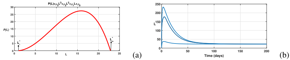
Figure 2 – Illustration of theorem 3 for 1 < \mathcal{N}^* = 61.4689 > \mathcal{N}_c = 13.144 and \Lambda_1 = 33 < \Lambda_1^{crit} = 164.31766 . So, the positive equilibrium Q_2^+ is locally stable.
