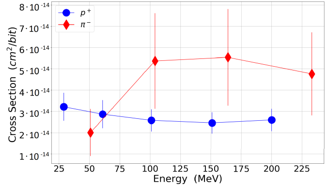
Fig. 3. Pion and proton SEU cross section for the Atmel SRAM with 95% confidence level error bars.
