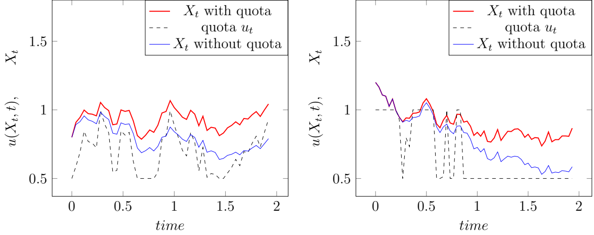
Figure 16: Optimal biomass and quota function computed by Optimal Control and compared with the solution with u = u_M when X_0 = 0.8 . Figure 17: Optimal biomass and quota function computed by Optimal Control and compared with the solution with u = u_M when X_0 = 1.2 .
