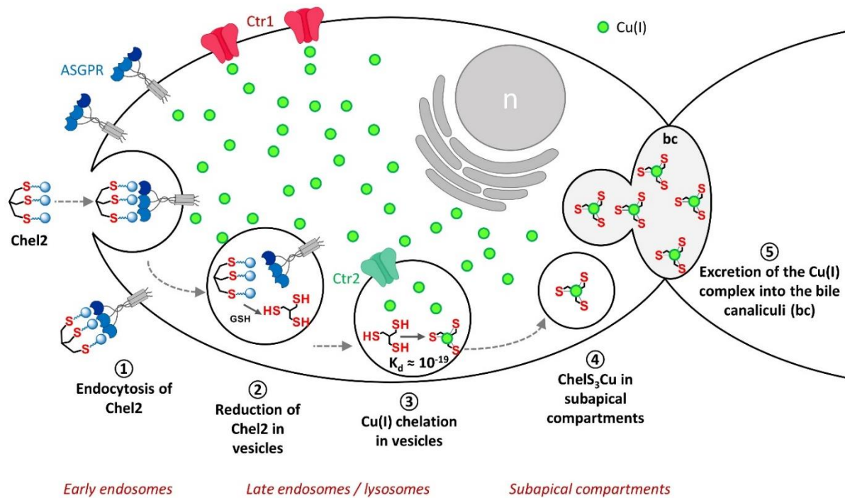
Scheme 2 Proposed mechanism for Chel2 fate in hepatic cells in the presence of Cu.
