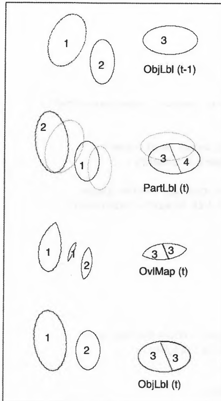
Figure 7.13 Steps involved to build the object label mask ObjLbl at time t from the object label mask at time t-1 and the particle label mask at time t. OvMap(t) represents the overlap between the particles at time t and the objects at time t-1. The numbers represent the labels of the objects.
