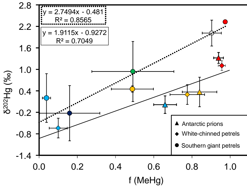
Figure S1. Hg MDF signatures (as \delta^{202}\text{Hg} ) relative to the percentage of MeHg for the three seabird species together. Mean values of feathers, muscles and livers of Antarctic prions ( n=10 ) and white-chinned petrels ( n=10 ) exhibited a regression line of y = 1.91x - 0.92 , Spearman correlation coefficients were R^2 = 0.70 , p < 0.0001 ; while the mean values of tissues of giant petrels ( n=3 ) exhibited a regression line of y = 2.75x - 0.48 , Spearman correlation coefficients were R^2 = 0.85 , p < 0.0001 . Highlighted symbols with error bars represent mean \pm SD values for each tissue.
