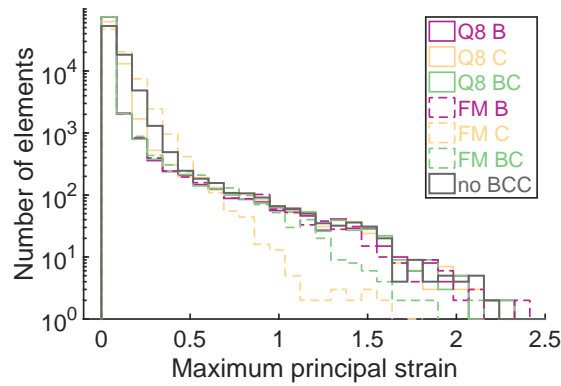
Figure 11: Histograms of maximum principal strain (dimensionless) for all BCC procedures using the last image of the experiment
