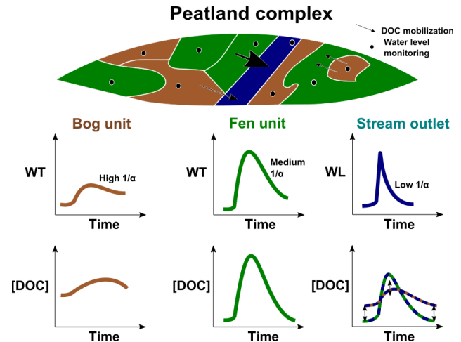
Figure 6. Schematic overview of a peatland complex. Size of the arrows corresponds to DOC quantity mobilized from distinct peatland units. The DOC concentration observed in the stream depends on the contribution of the different peat units within the peatland complex.
