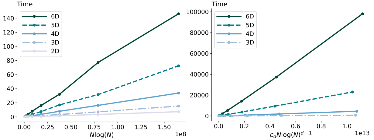
Figure 4: Runtime for KDE estimation (left: fast summation; right: divide-and-conquer)
