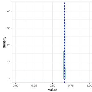
(C) Histogram of system's ( N = 30 ) components values from 100 (independent) samples, at time N = 2 computed using the software Mathematica 5.000. Starting conditions are always 1/2 .
