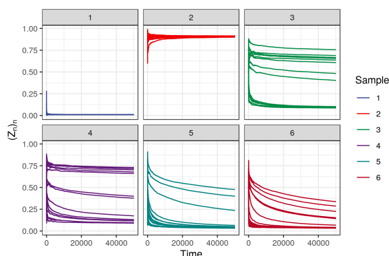
(A) Six samples of the system's trajectories when N = 15 . Each system starts at 1/2 on the diagonal.
