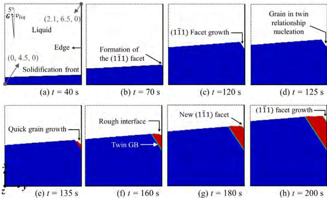
Fig. 12. 3D CA computations showing (a) growth of a solidification front from an initial seed, (b) formation of a (111) facet, (c) growth of the facet, (d) nucleation of a grain in twin relationship at the bottom of the facet, (e) quick twin growth along the (111) facet defining the twin grain boundary, (g) twin growth and formation of a new (111) facet and (h) growth of the new (111) facet. The blue and red grains are in Σ3 twin relationship. Coordinates of the bottom-left and top-right corners are given in mm. See Table 1 for simulation parameters.
