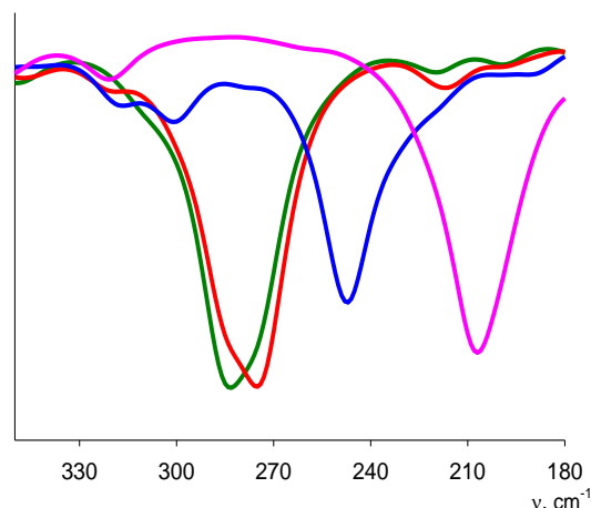
Figure 5. Calculated IR spectra (lower fingerprint region) of 1^{\text{Bu}} type I (green line), 1^{\text{Ph}} type I (red line), 1^{\text{Bu}} type II' (pink line) and 1^{\text{Ph}} type II' (blue line).
