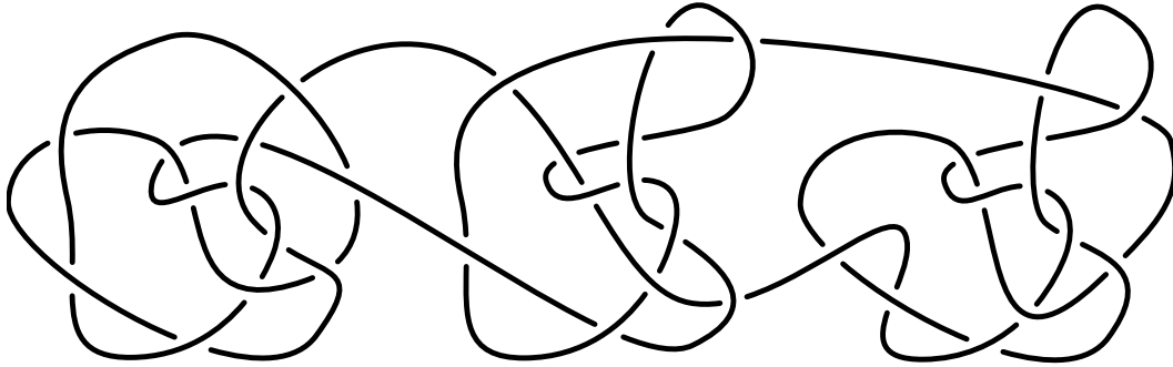
Figure 3 – This figure represents the knot \#(\gamma, 3) . As \gamma (figure 1) is 3-trivial, this one is 9-trivial. Cette figure représente le noeud \#(\gamma, 3) . Comme \gamma (figure 1) est 3-trivial, celui-ci est 9-trivial.
