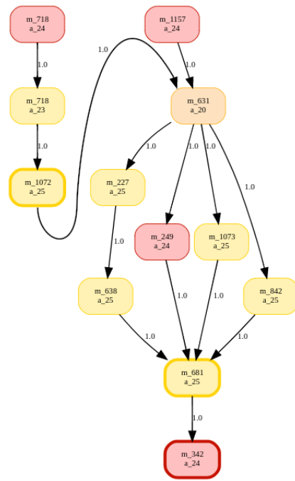
Fig. 3. Most relevant sequences of alarms starting by a severe (red) alarm and ending by an active (bold) severe alarm (edge weights correspond to a causal relevance quantified by ratios introduced in [4])
