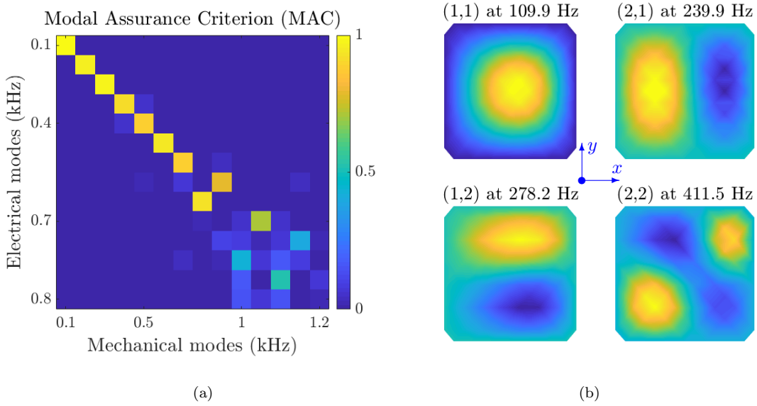
Figure 18: (a) MAC matrix between simulated electrical current modes of the network and simulated velocity modes of the variable thickness plate. (b) First four modes of the variable thickness plate electrical analogous network.
