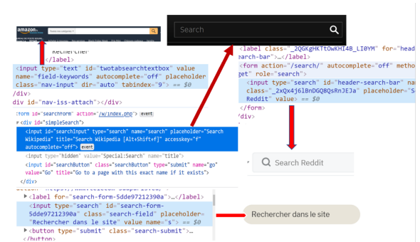
Figure 5: SVM model detects search box pattern.
