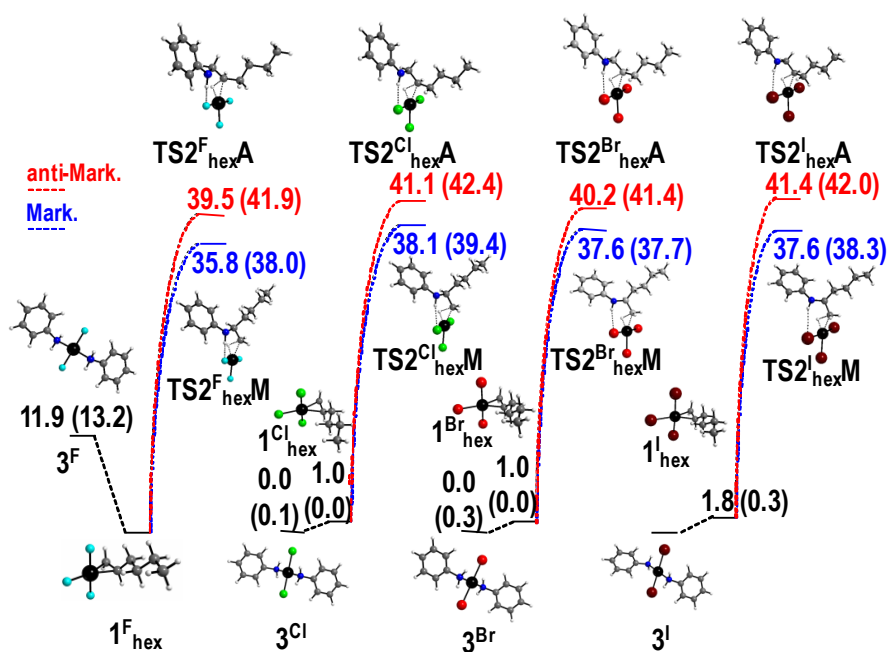
Figure 12. Relative Gibbs free energies for systems [\text{PtX}_3(1\text{-hexene})]^- ( \mathbf{1}^{\text{X}_{\text{hex}}} ), \text{trans-PtX}_2(\text{PhNH}_2)_2 ( \mathbf{3}^{\text{X}} ) and the transition states of the rate determining C-H reductive elimination steps ( \text{TS2}^{\text{X}_{\text{hex}}} ) for both Markovnikov and anti-Markovnikov products related to the \text{PtX}_2/\text{X}^- catalyzed hydroamination of 1-hexene. Values are \Delta G^{\text{CPCM}} (aniline) in \text{kcal mol}^{-1} relative to the resting state in each case, at 298.15 K (and at 423.15 K in parentheses).
