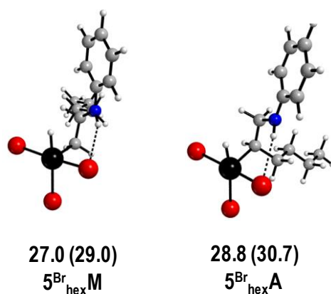
Figure 9. Geometries and relative Gibbs free energies of the Pt IV hydride intermediates 5^{\text{Br}}_{\text{hexM}} and 5^{\text{Br}}_{\text{hexA}} . Values are \Delta G^{\text{CPCM}} (aniline) in kcal mol -1 relative to [PtBr 3 (1-hexene)] - ( 1^{\text{Br}}_{\text{hex}} ) at 298.15 K (and at 423.15 K in parentheses).
