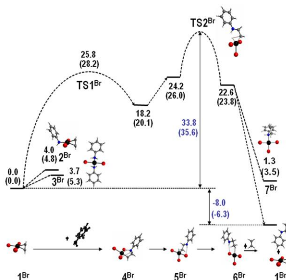
Figure 1. Free energy profile of the aniline addition to ethylene catalyzed by \text{PtBr}_2/\text{Br}^- . 39 Values are \Delta G^{\text{CPCM}} (aniline) relative to [\text{PtBr}_3(\text{C}_2\text{H}_4)]^- in \text{kcal mol}^{-1} at 298.15 K (and at 423.15 K in parentheses).
