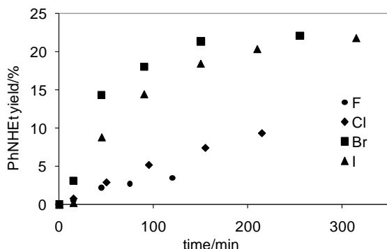
Figure 4. Kinetic profiles of the hydroamination of C_2H_4 by aniline, catalyzed by PtBr_2/nBu_4PX ( X = Cl, Br, I ) or PtBr_2/nBu_4NF \cdot 3H_2O . Conditions: PtBr_2 , 0.26 mmol; salt additive, 2.6 mmol; PhNH_2 , 90 mmol; p(C_2H_4) = 25 bar at 298K (ca. 100 mmol), 150°C.
