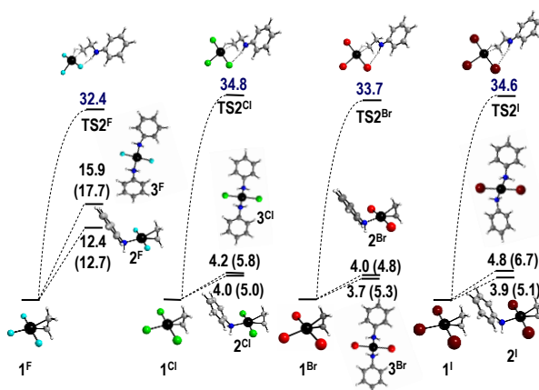
Figure 2. Relative Gibbs free energies of [\text{PtX}_3(\text{C}_2\text{H}_4)]^- ( \mathbf{1}^{\text{X}} ), trans - \text{PtX}_2(\text{C}_2\text{H}_4)(\text{PhNH}_2) ( \mathbf{2}^{\text{X}} ), trans - \text{PtX}_2(\text{PhNH}_2)_2 ( \mathbf{3}^{\text{X}} ), and the TOF-determining transition state ( \text{TS2}^{\text{X}} ) for the ethylene/aniline process. Values are \Delta G^{\text{CPCM}} (aniline) relative to \mathbf{1}^{\text{X}} in kcal mol -1 at 298.15 K (and at 423.15 K in parentheses).
