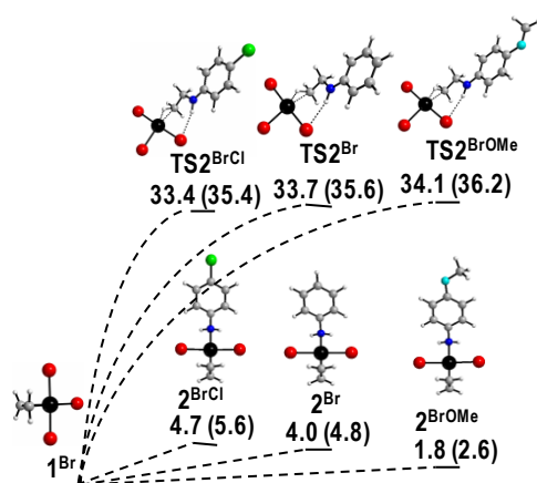
Figure 5. Relative Gibbs free energy of the trans -PtBr 2 (C 2 H 4 )(ArNH 2 ) (Ar = 4-C 6 H 4 OMe, 2 BrOMe ; C 6 H 5 , 2 Br ; 4-C 6 H 4 Cl, 2 BrCl ) and the corresponding TOF-determining transition states ( TS2 BrOMe , TS2 Br , TS2 BrCl ). Values are \Delta G_{\text{cycle}}^{\text{CPM}} (aniline) relative to [PtBr 3 (C 2 H 4 )] - ( 1 Br ) in kcal mol -1 at 298.15 K (and at 423.15 K in parentheses).
