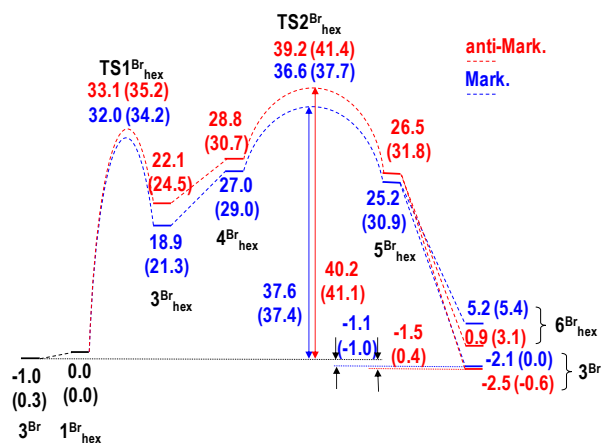
Figure 11. Relative Gibbs free energy pathways for the PtBr 2 /Br - catalyzed hydroamination of 1-hexene. Values are \Delta G^{\text{CPCM}} (aniline) in kcal mol -1 relative to [PtBr 3 (1-hexene)] - ( \mathbf{1}^{\text{Br}}_{\text{hex}} ) at 298.15 K (and at 423.15 K in parentheses).
