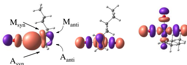
Figure 7. Three mutually orthogonal views of the LUMO ( E = 0.0424 Hartree) of complex \mathbf{1}^{\text{Br}}_{\text{hex}} , with indication of all possible pathways for nucleophilic aniline addition.
