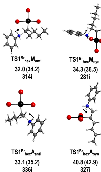
Figure 8. Views of the lowest energy transition states for the four types of nucleophilic addition of \text{PhNH}_2 to coordinated 1-hexene in \mathbf{1}^{\text{Br}}_{\text{hex}} . Values of \Delta G^{\text{CPCM}} (aniline) in \text{kcal mol}^{-1} relative to [\text{PtBr}_3(1\text{-hexene})]^- ( \mathbf{1}^{\text{Br}}_{\text{hex}} ) at 298.15 K (and at 423.15 K in parentheses) and of the calculated imaginary frequency in \text{cm}^{-1} are also shown.
