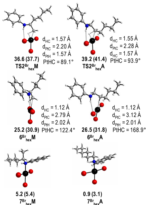
Figure 10. Geometries and relative Gibbs free energies of the transition states and products, TS2 Br hex and 6 Br hex , of the C-H reductive elimination from the hydride complexes 5 Br hex , as well as of the products of rearrangement of the N -1- or N -2-hexylaniline, 7 Br hex . Values are \Delta G^{\text{CPCM}} (aniline) in kcal mol -1 relative to [PtBr 3 (1-hexene)] - ( 1 Br hex ) at 298.15 K (and at 423.15 K in parentheses).
