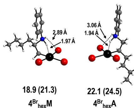
Figure 6. Geometries and relative Gibbs free energies of the most stable products of PhNH 2 addition to the CHBr ( 4 Br hex M ) and CH 2 ( 4 Br hex A ) groups of the coordinated 1-hexene in [PtBr 3 (1-hexene)] - ( 1 Br hex ). Values are \Delta G^{\text{CPCM}} (aniline) in kcal mol -1 relative to 1 Br hex at 298.15 K (and at 423.15 K in parentheses).
