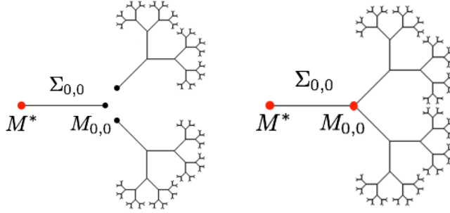
FIGURE 2. Left: we illustrate the space \tilde{V}_{\mathfrak{n}}(\mathcal{T}) , which includes functions that may be discontinuous in the point M_{0,0} . Right: an illustration to the space \tilde{V}_{\mathfrak{n},0}(\mathcal{T}) , where all functions vanish in the point M_{0,0} . By red we mark the points where the functions vanish.
