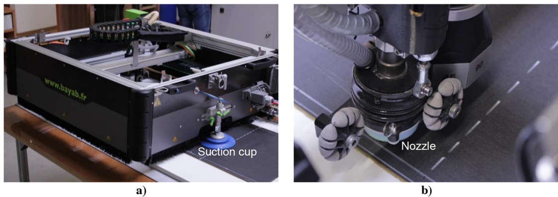
Fig. 4. Abrasive water jet machine Reply.5 with (a) levelled machine and (b) nozzle.
