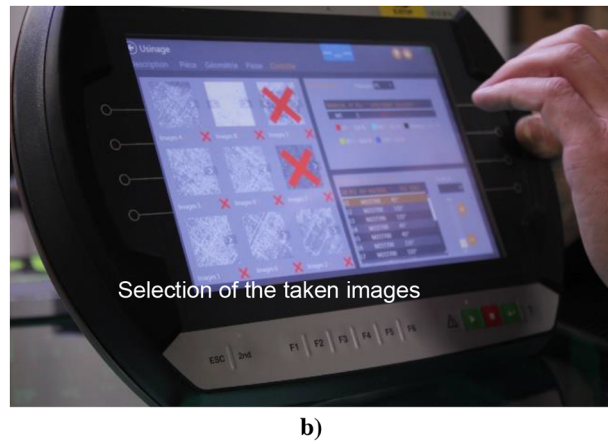
Fig. 7. Verification process of the machining surface with (a) overlap zone analysed by image analysis and (b) visualization and selection of the images on the control panel to estimate the location of the interface between to plies (i.e. presence of numerous dark spots due to no light diffraction).
