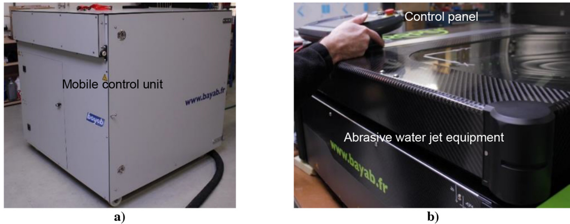
Fig. 3. Bayab Industries abrasive water jet machine REPLY.5 with (a) control unit and (b) abrasive water jet equipment (50 kg) and control panel.
