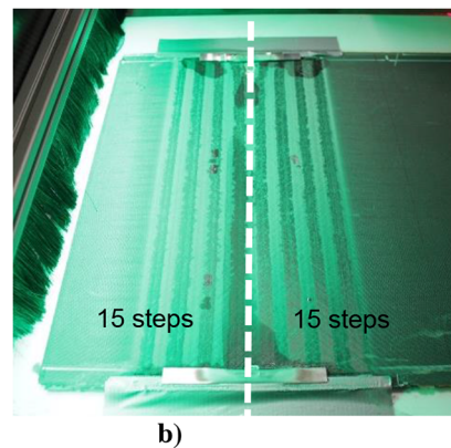
Fig. 8. Machining of the 15 steps (for 16 plies in total) with (a) scheme of milled profile (not to scale) and (b) view of the finished milled stepped-lap for the overlap ratio of 20.
