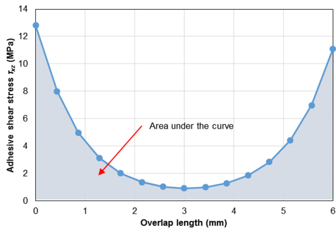
Fig. 23. Determination of the average shear value along the adhesive joint for 6 mm overlap length [7].
