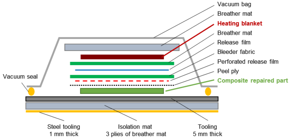
Fig. 11. Scheme of the vacuum bag products (not to scale) for the composite patch curing by heating blanket (according to SRM A350 chapter 51.77.11, see [6]).
