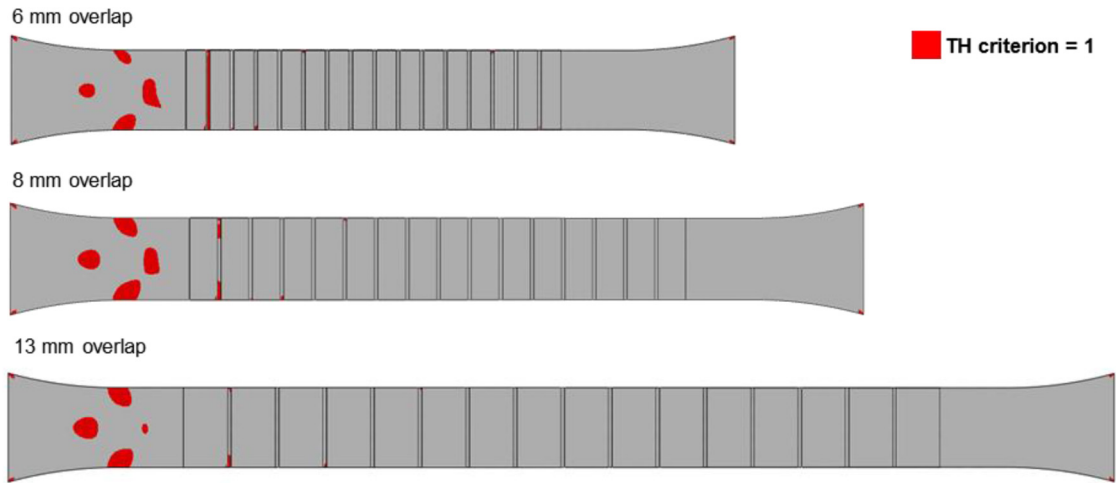
Fig. 21. Tsai-Hill criterion (TH = 1 in red when the chosen limit values are reached) in the FE models for the 6, 8 and 13 mm overlap lengths (from top to bottom).
