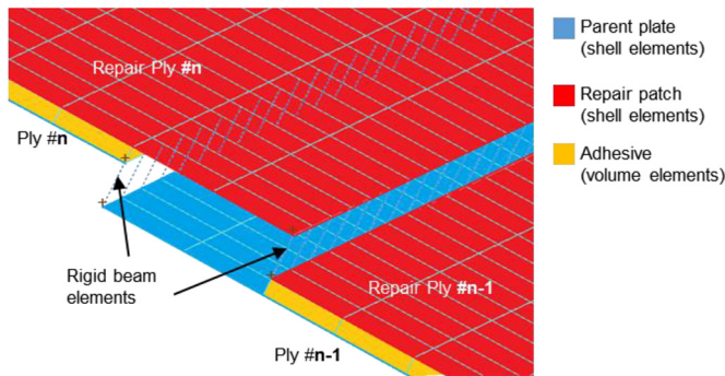
Fig. 15. Mesh detail between two consecutive steps (ply #n and #n-1).
