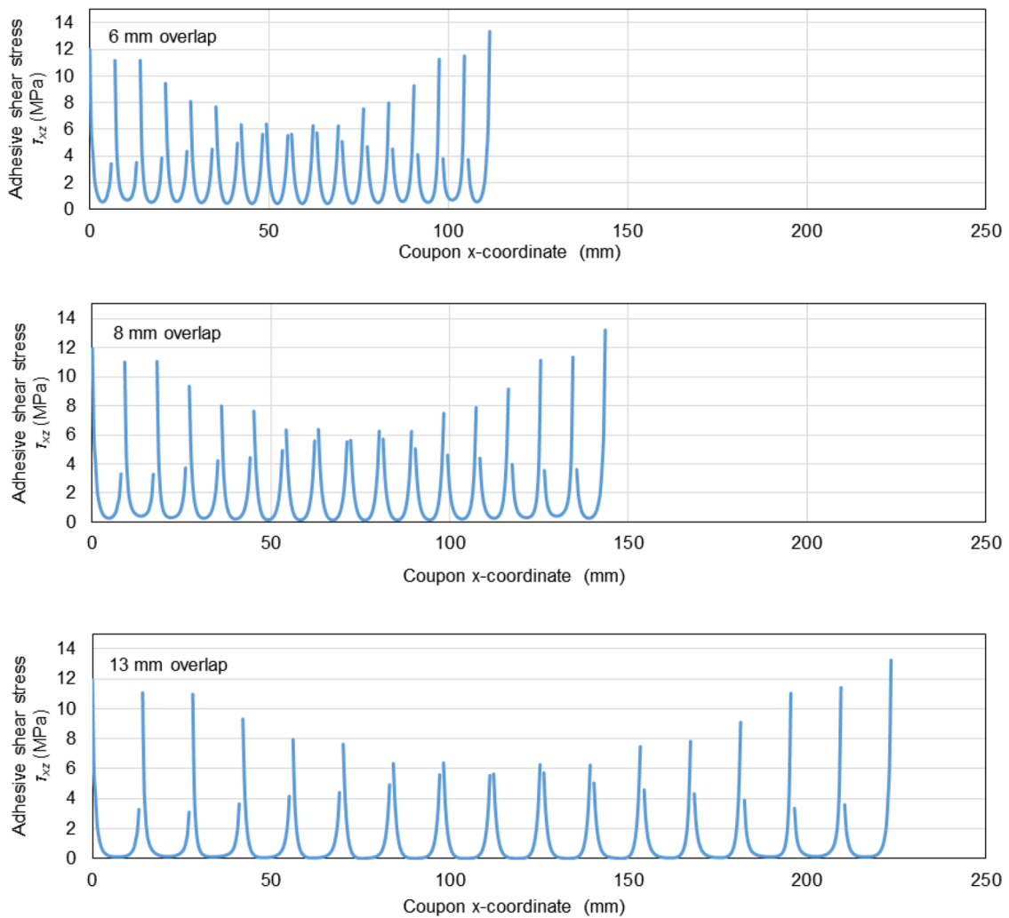
Fig. 22. Shear stress \tau_{xz} distribution in the adhesive in each step (from top to bottom) for the 6, 8 and 13 mm overlap lengths.
