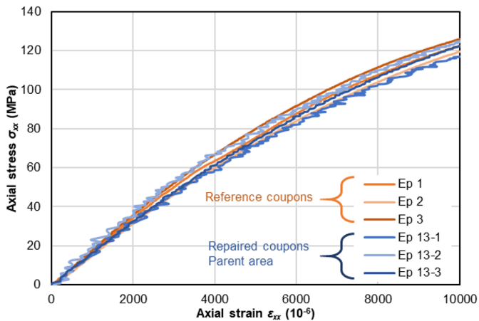
Fig. 20. Axial stress \sigma_{xx} – strain \epsilon_{xx} curve of the parent area of repair coupons Ep 13-1, 13-2 and 13-3 and reference test coupons Ep 1, 2 and 3.
