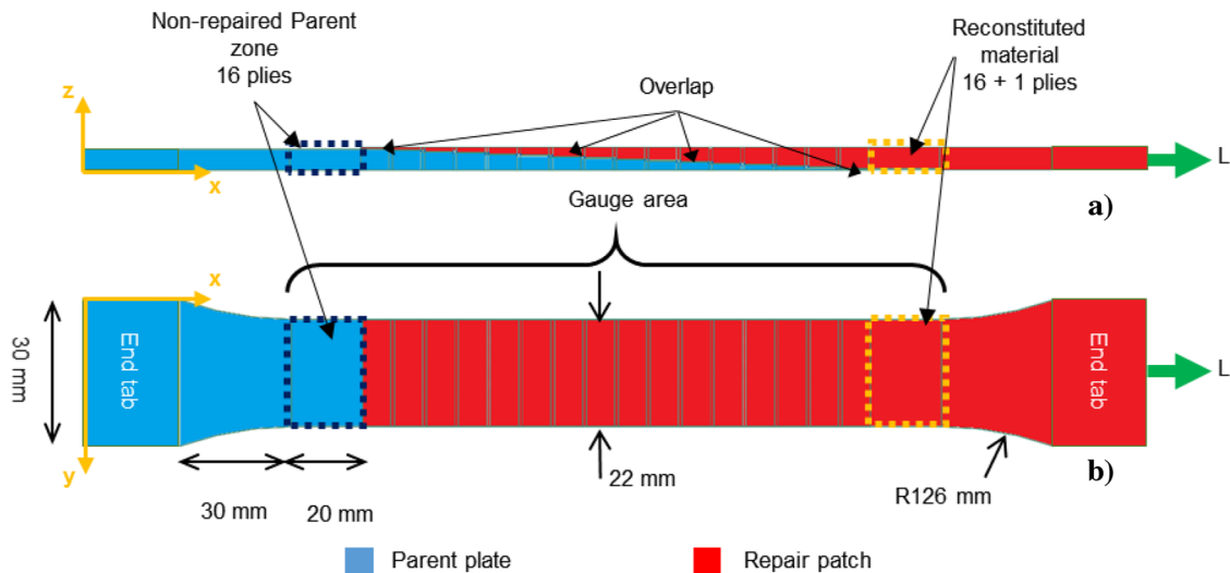
Fig. 16. 3D representation of the FE model (shell thicknesses rendered at their given values) with (a) side view (XZ plane) and (b) top view (XY plane).
