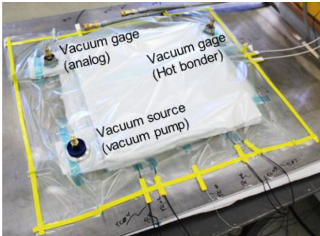
Fig. 12. Overview of the vacuum bag products and the connections to the different thermocouples.
