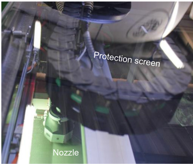
Fig. 6. View through the protection screen of the machine during the machining of the step #1 for the stepped lap ratio of 1:20 (step length over ply thickness).
