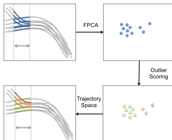
Figure 1: Illustration of the methodology for detecting atypical trajectories. A sliding window is applied on all trajectories. The dimension is then reduced by applying a Functional Principal Component Analysis decomposition on the portions of such trajectories. An outlier detection and scoring is applied on the decomposition vector space, which allows to assign to each trajectory portion a score between 0 and 1, determining the local atypicality.
