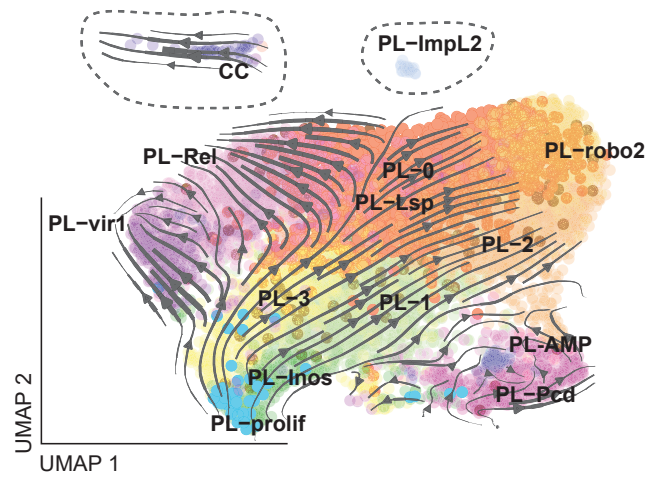
C Lineage prediction (Velocity)
