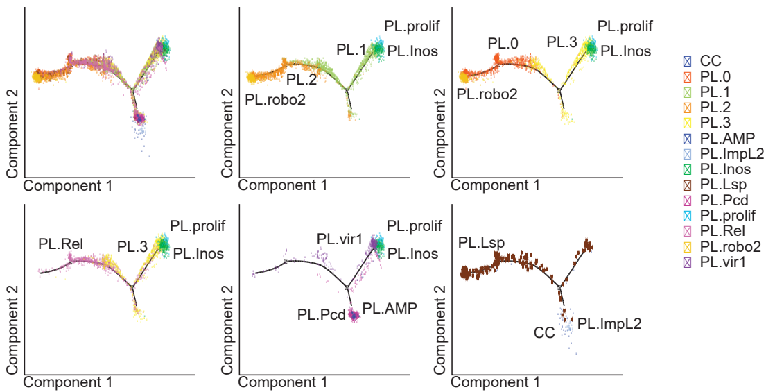
D Lineage prediction (Monocle 2)
