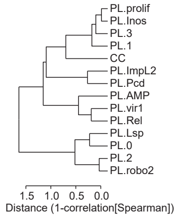
C Lineage prediction (Velocity)
