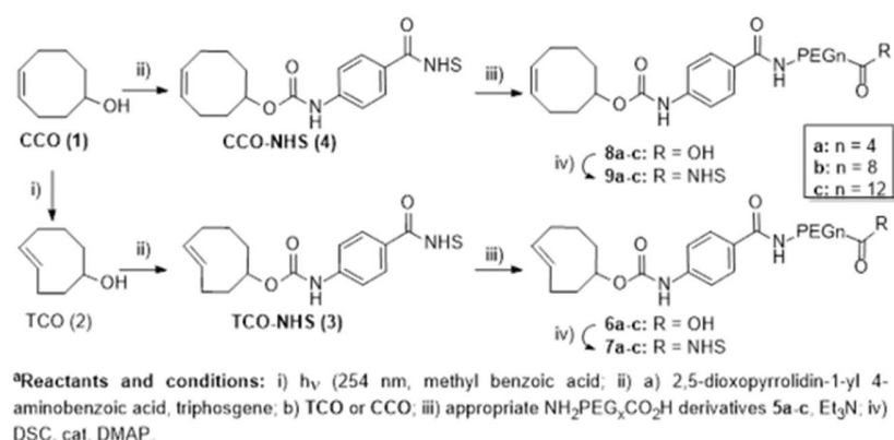
Scheme 1: TCO derivative syntheses with high TCO/CCO ratio
