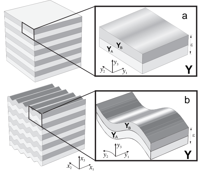
Fig. 1. Flexoelectric multilayered composite: a) rectangular geometry at the periodic cell and b) with complex geometrical shape microstructure.
