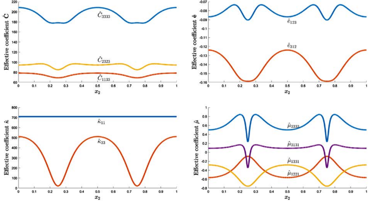
Fig. 3. Effective coefficients components \hat{C}_{3333} , \hat{C}_{2323} , \hat{C}_{1133} (stiffness), \hat{e}_{123} , \hat{e}_{312} (piezoelectric), \hat{\kappa}_{11} , \hat{\kappa}_{33} (relative effective permittivity) and \hat{\mu}_{3333} , \hat{\mu}_{3131} , \hat{\mu}_{1331} , \hat{\mu}_{1221} (flexoelectric).
