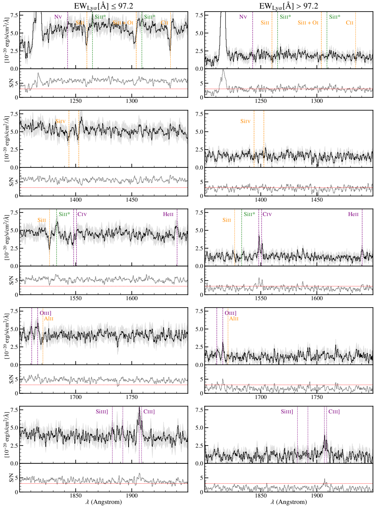
Fig. A.4. Mean spectra of LAEs with Ly \alpha EW [ \text{\AA} ] \leq 97.2 and >97.2 (left and right, respectively). The median values of the Ly \alpha EW for the two subsamples are 54.7 and 163.1, respectively. Lines and symbols as in Fig. 4.
